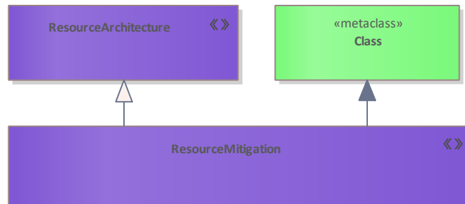
Figure 304: ResourceMitigation
