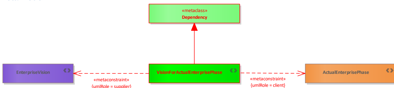
Figure 370: VisionForActualEnterprisePhase
