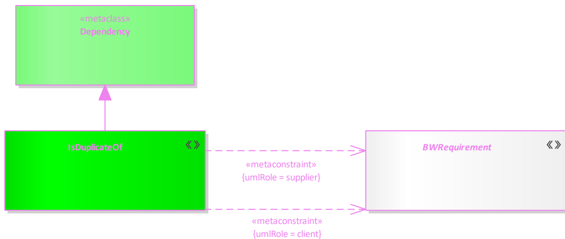
Figure 187: IsDuplicateOf
