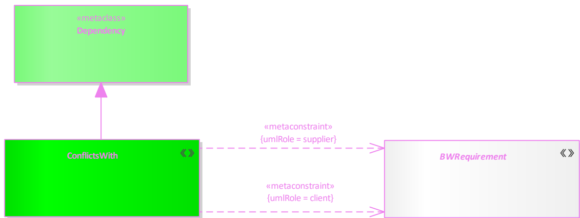
Figure 131: ConflictsWith
