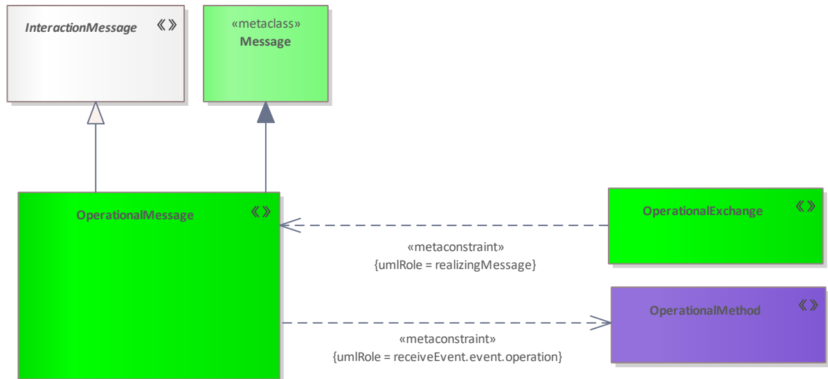
Figure 219: OperationalMessage
