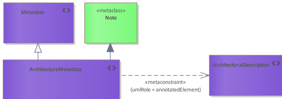
Figure 103: ArchitectureMetadata
