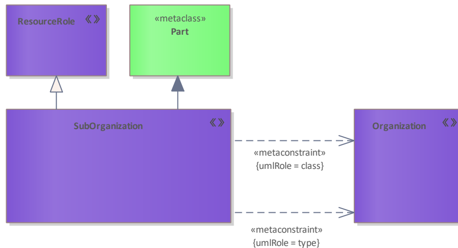
Figure 353: SubOrganization
