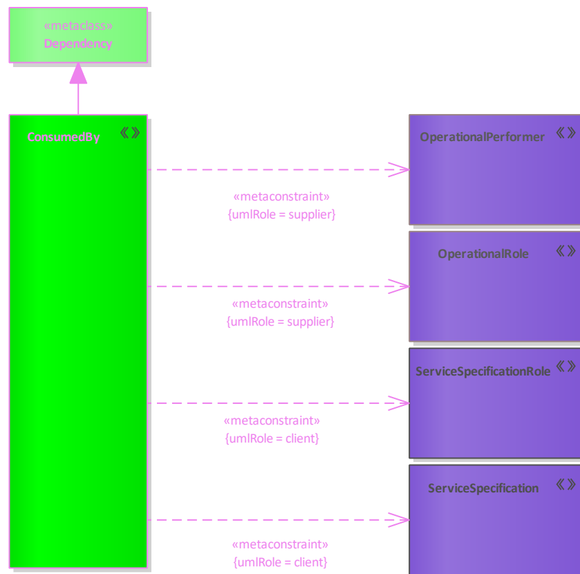
Figure 133: ConsumedBy
