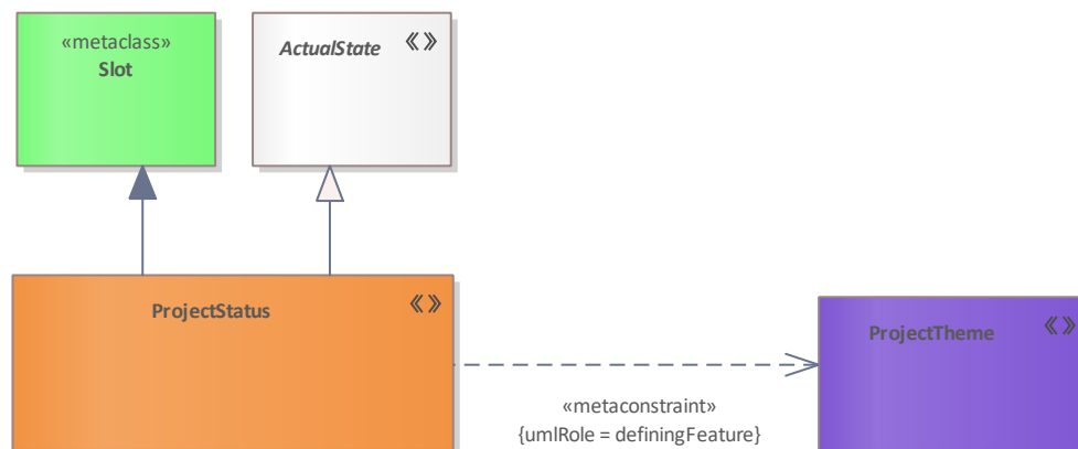
Figure 261: ProjectStatus
