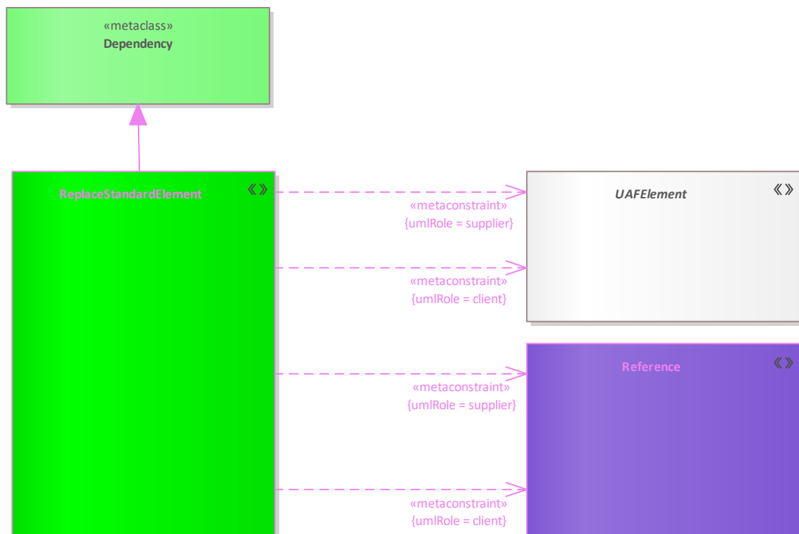
Figure 284: ReplaceStandardElement
