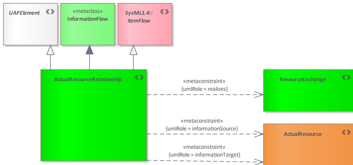
Figure 85: ActualResourceRelationship
