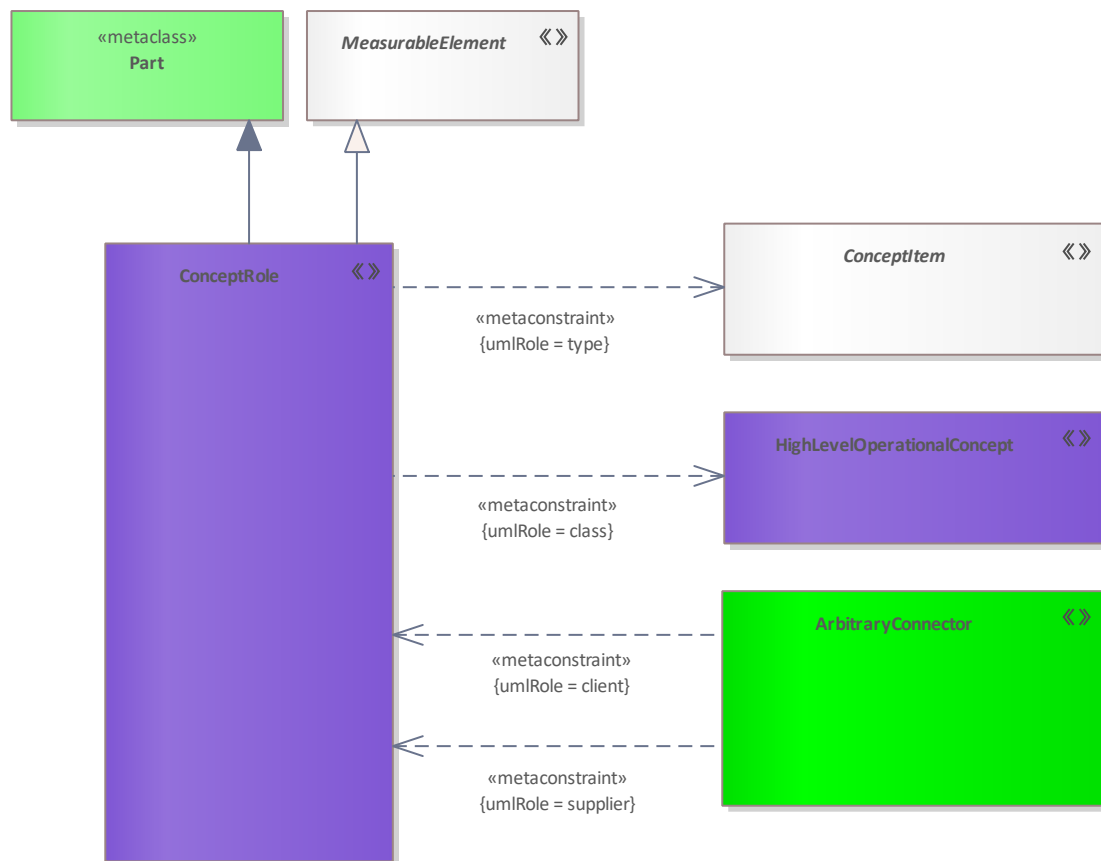
Figure 125: ConceptRole
