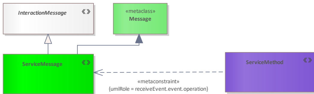
Figure 328: ServiceMessage
