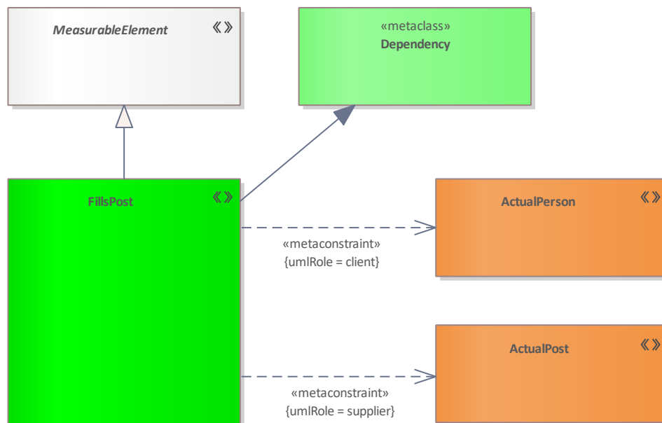
Figure 160: FillsPost
