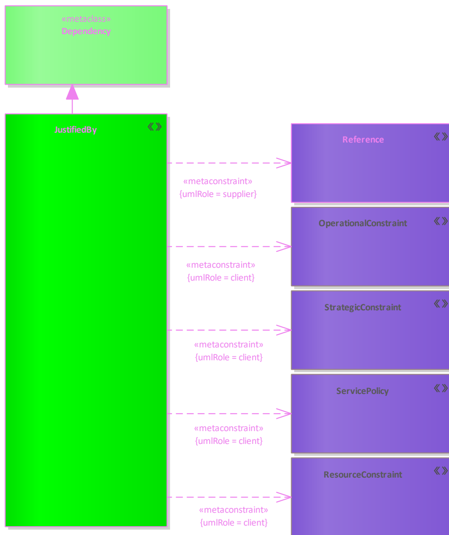
Figure 190: JustifiedBy
