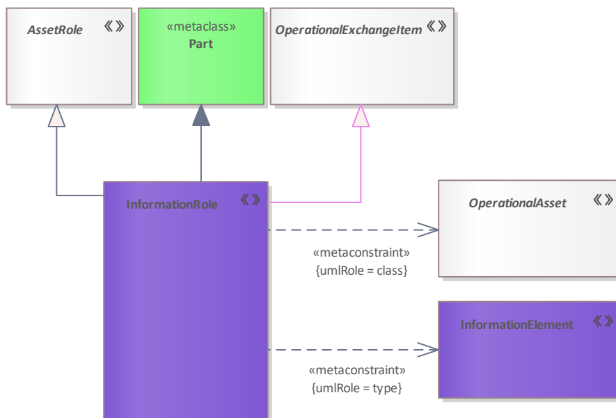
Figure 182: InformationRole
