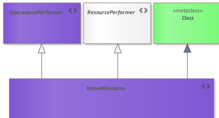
Figure 191: KnownResource
