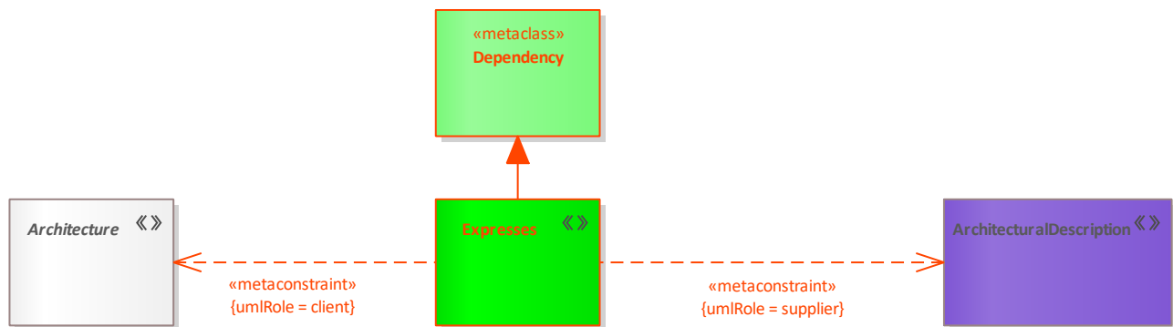
Figure 158: Expresses
