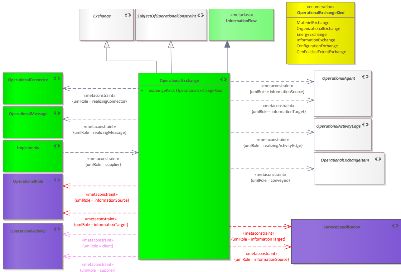
Figure 216: OperationalExchange
