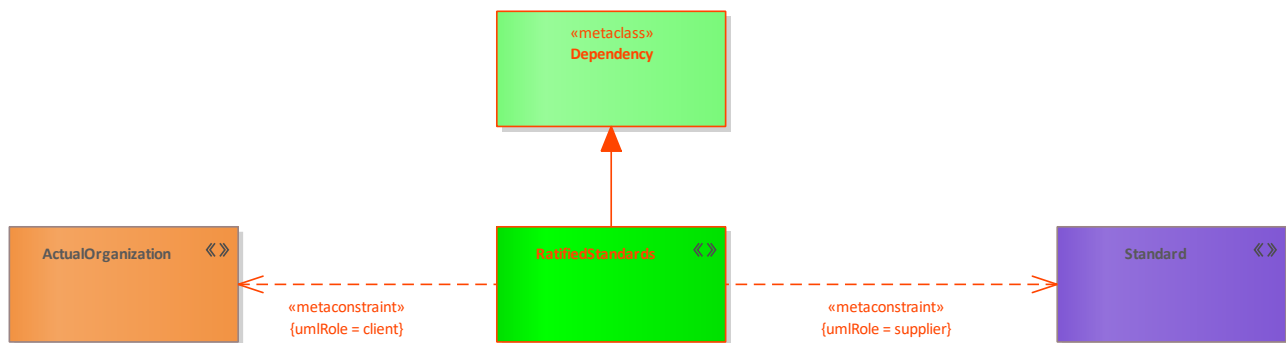
Figure 274: RatifiedStandards
