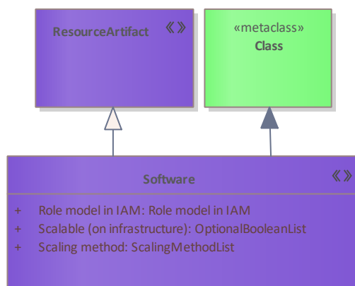
Figure 339: Software
