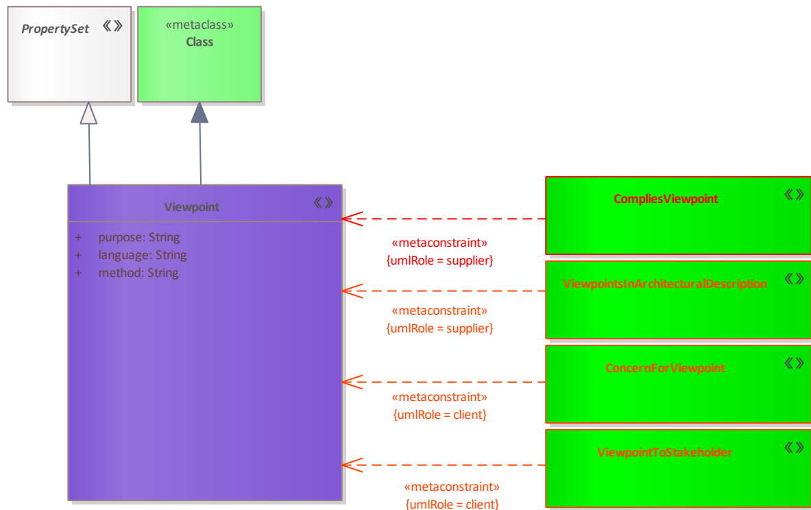
Figure 366: Viewpoint
