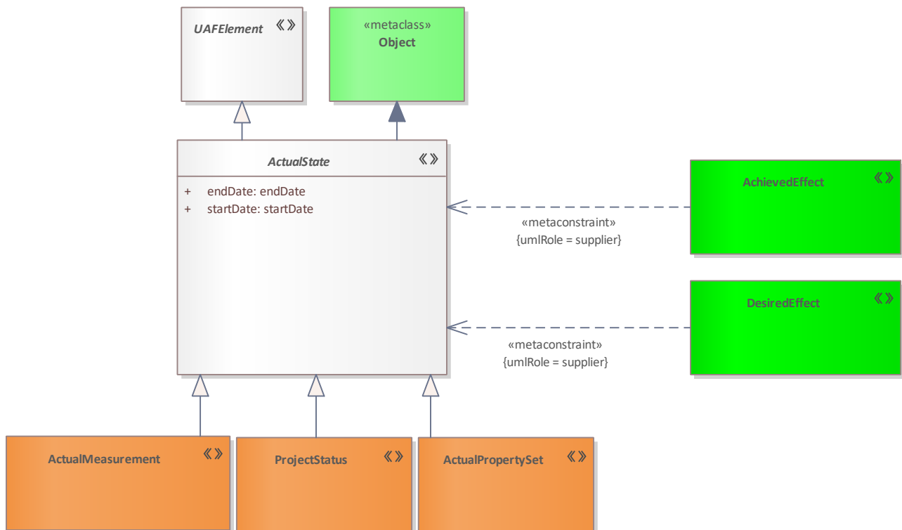
Figure 91: ActualState
