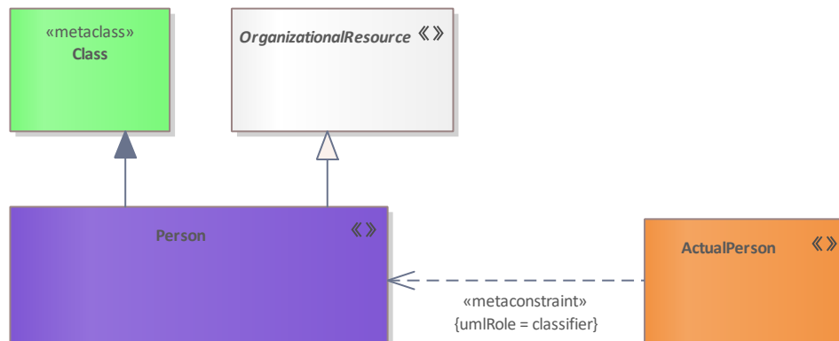
Figure 241: Person
