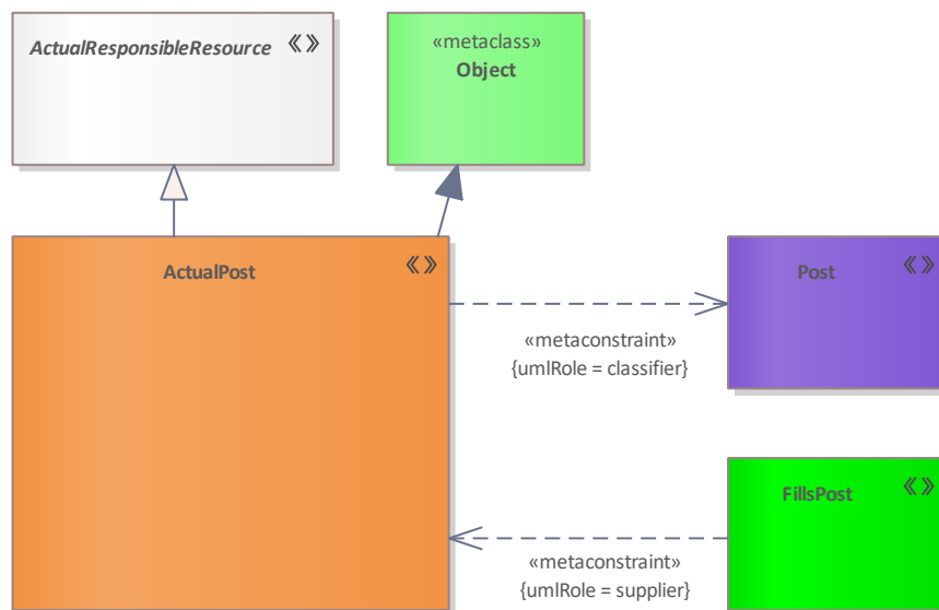
Figure 75: ActualPost
