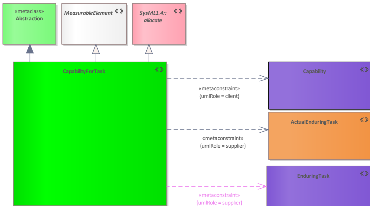
Figure 112: CapabilityForTask
