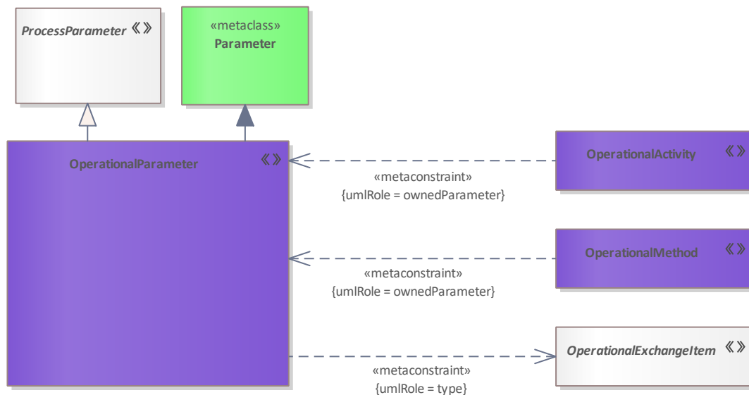
Figure 223: OperationalParameter
