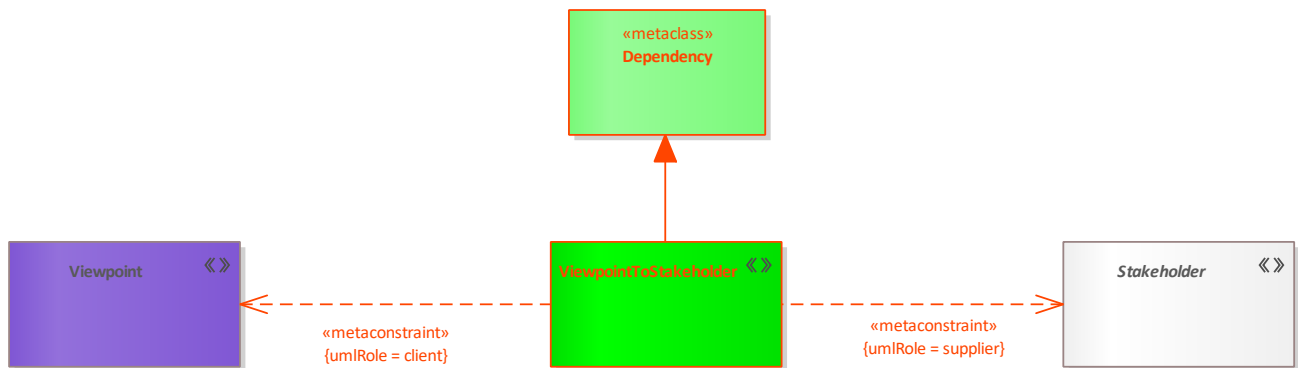
Figure 368: ViewpointToStakeholder
