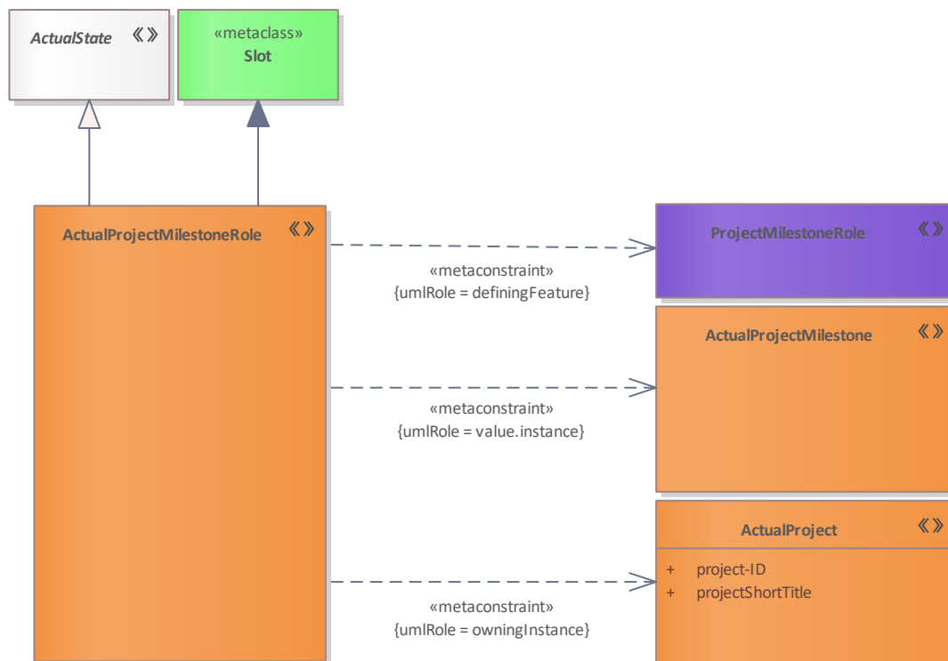
Figure 81: ActualProjectMilestoneRole
