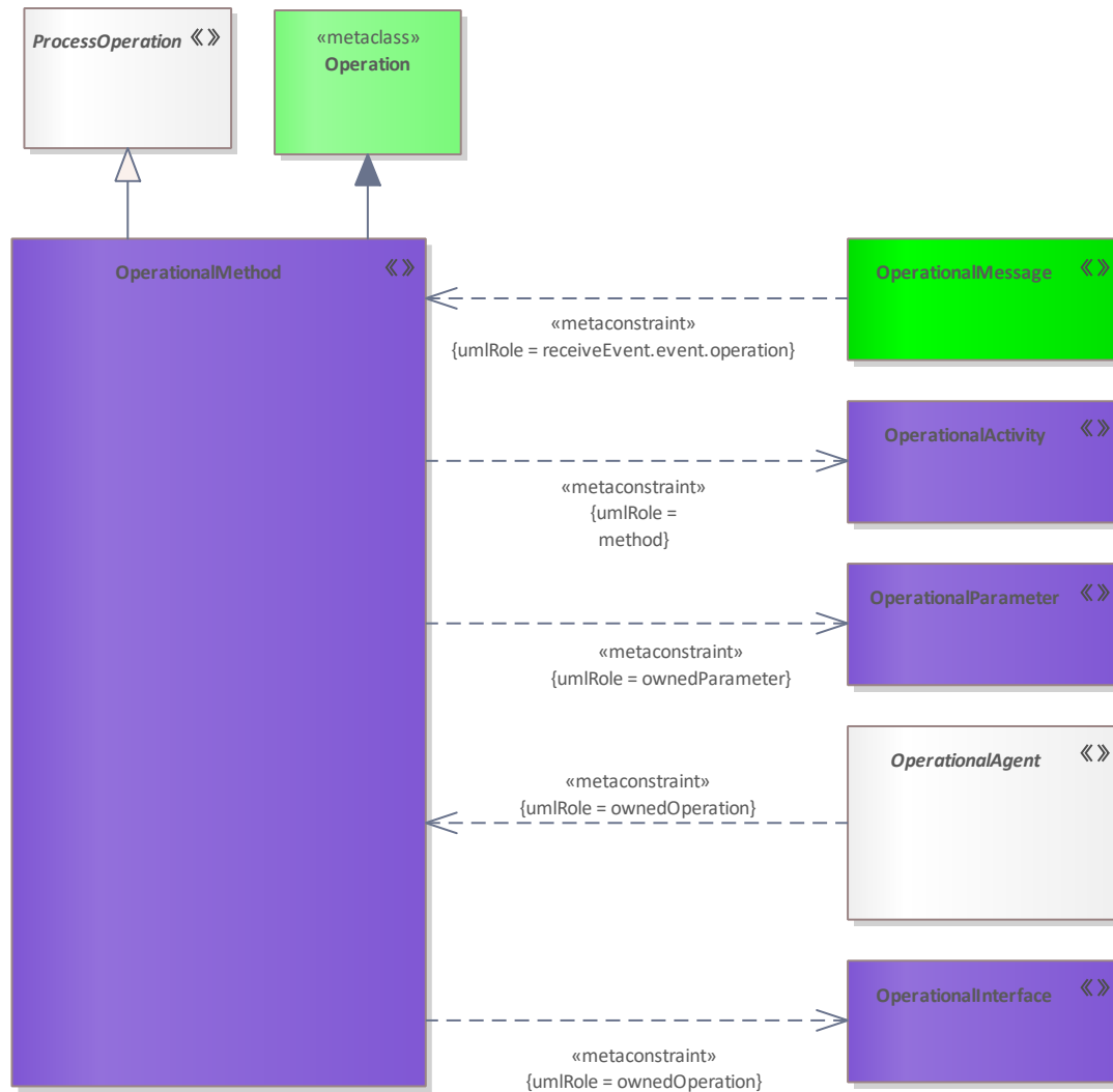
Figure 221: OperationalMethod
