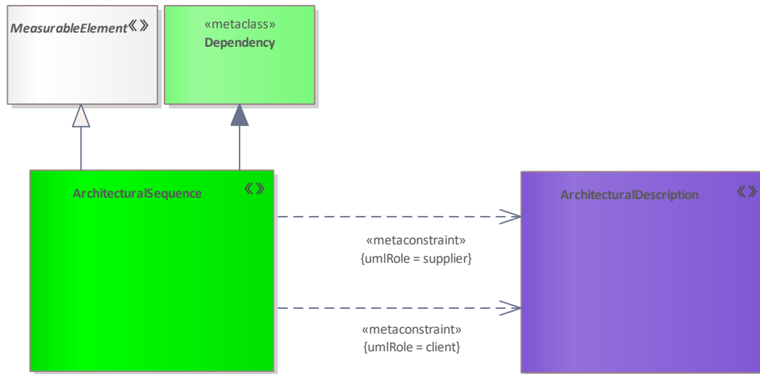
Figure 100: ArchitecturalSequence
