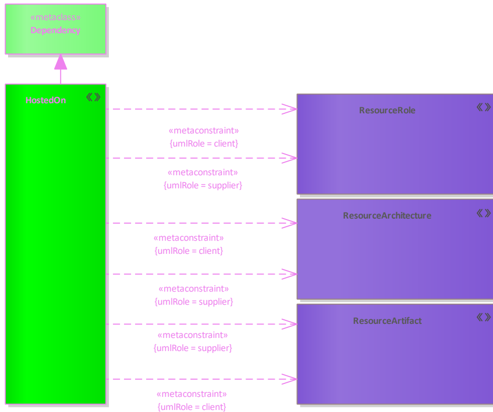
Figure 177: HostedOn
