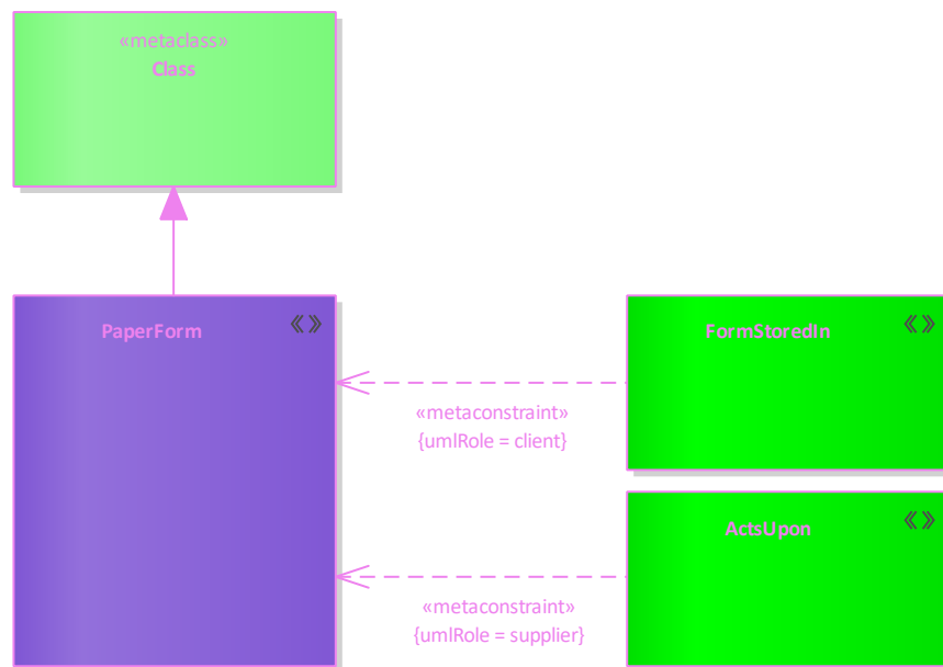
Figure 237: PaperForm
