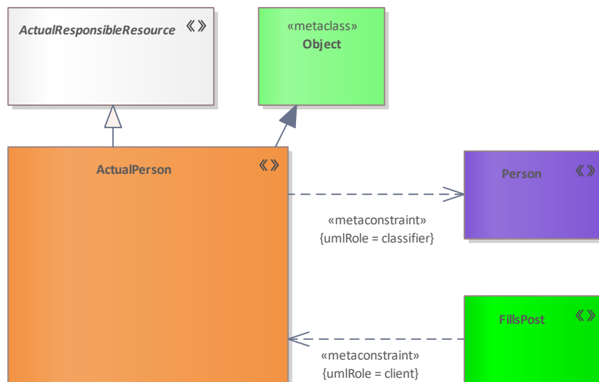
Figure 74: ActualPerson
