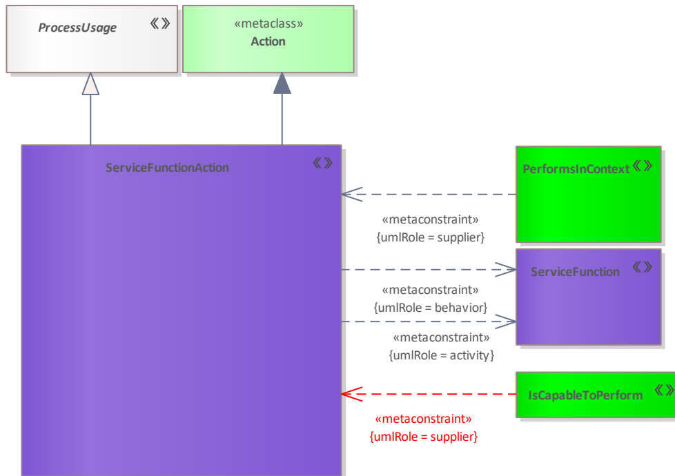
Figure 326: ServiceFunctionAction
