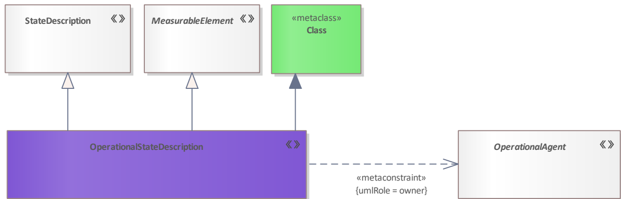
Figure 229: OperationalStateDescription
