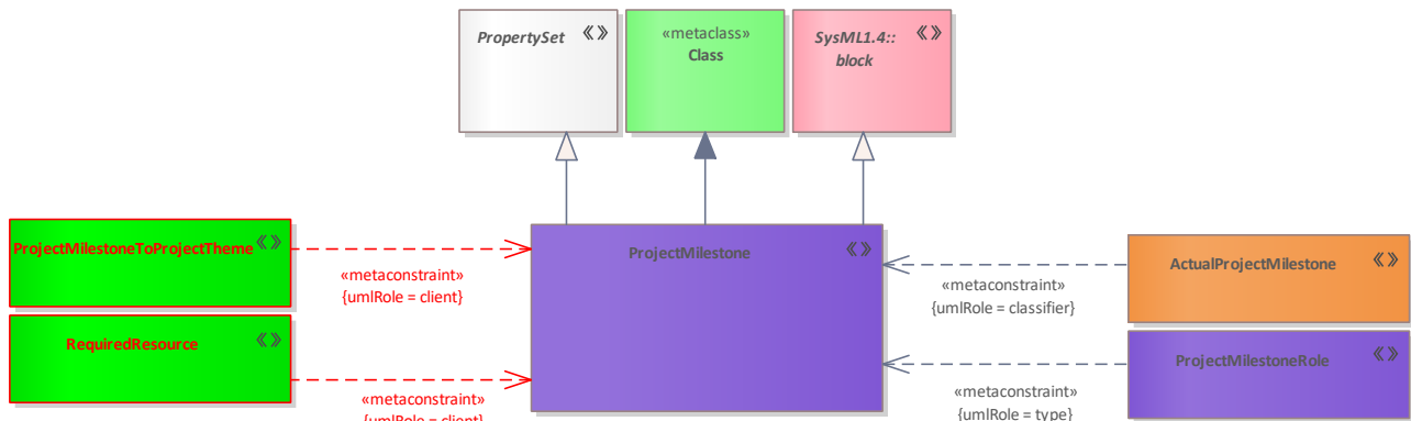
Figure 255: ProjectMilestone
