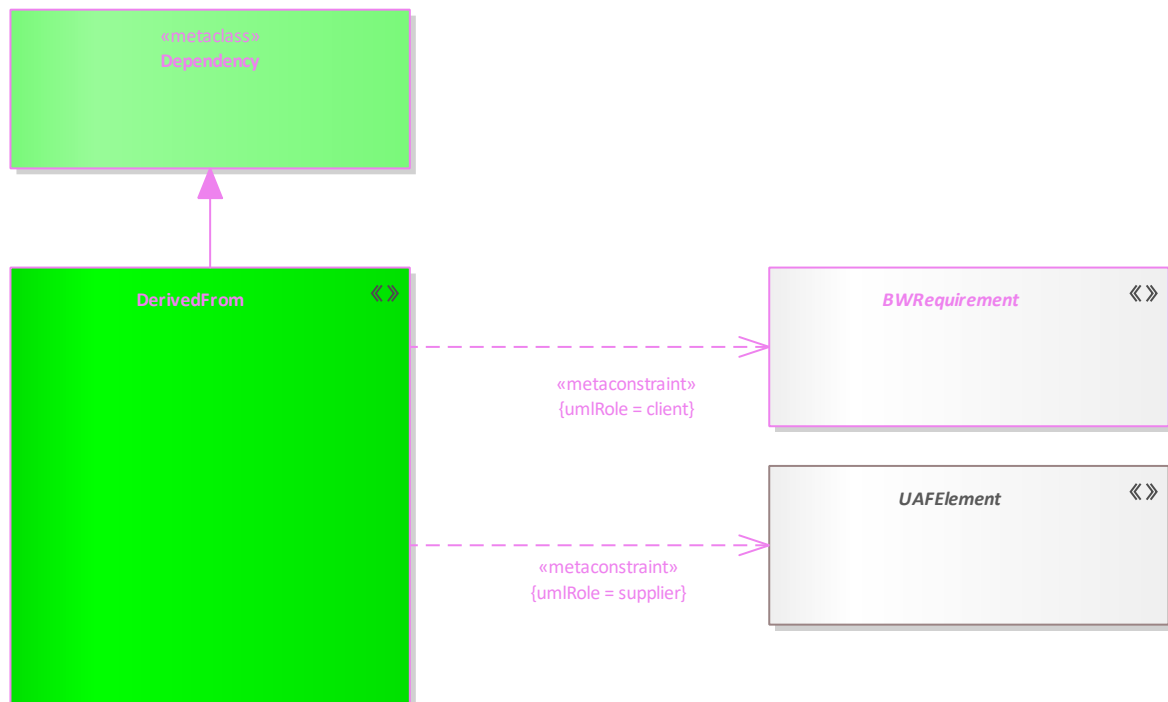
Figure 140: DerivedFrom
