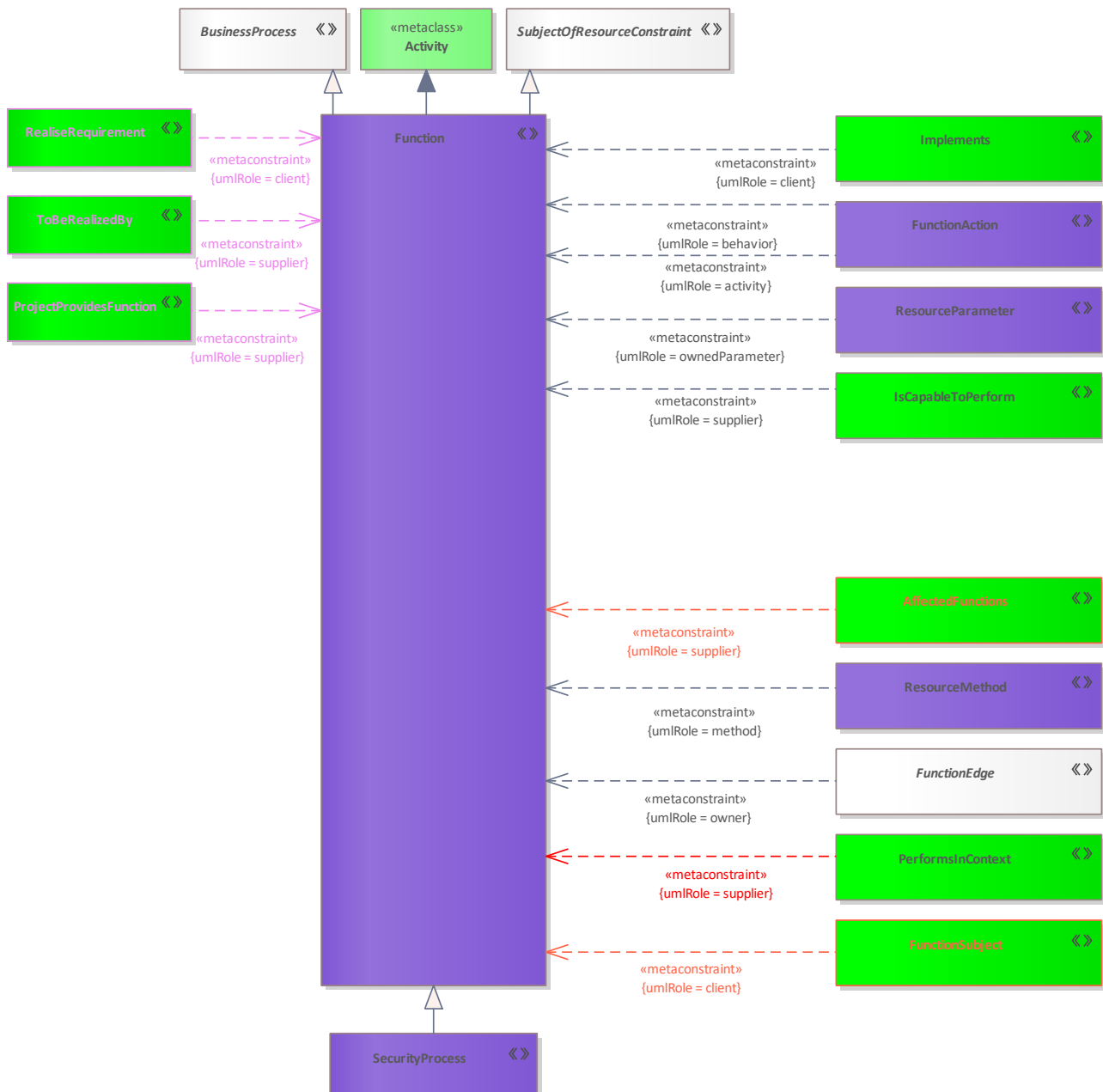
Figure 167: Function
