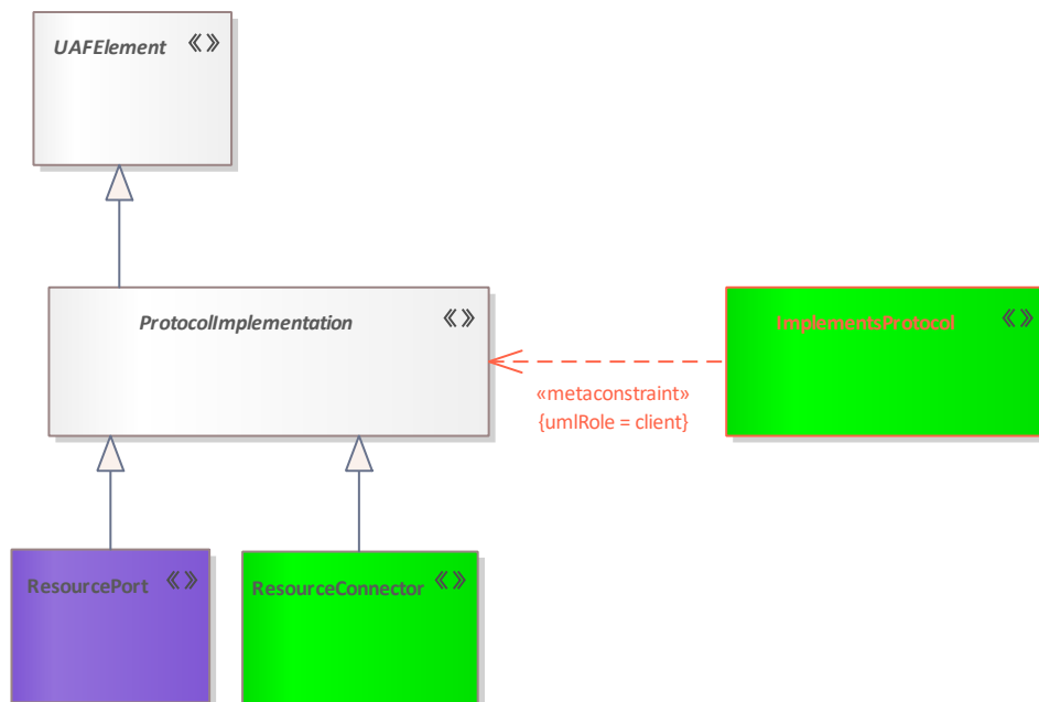
Figure 267: ProtocolImplementation
