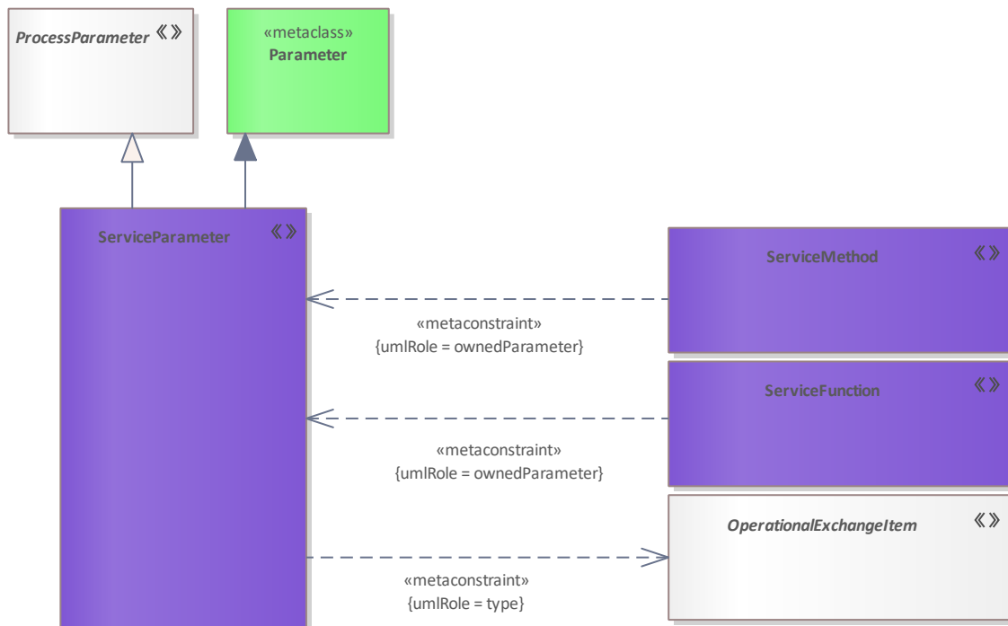
Figure 330: ServiceParameter
