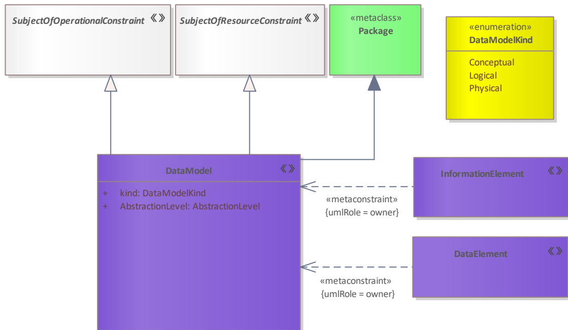
Figure 137: DataModel
