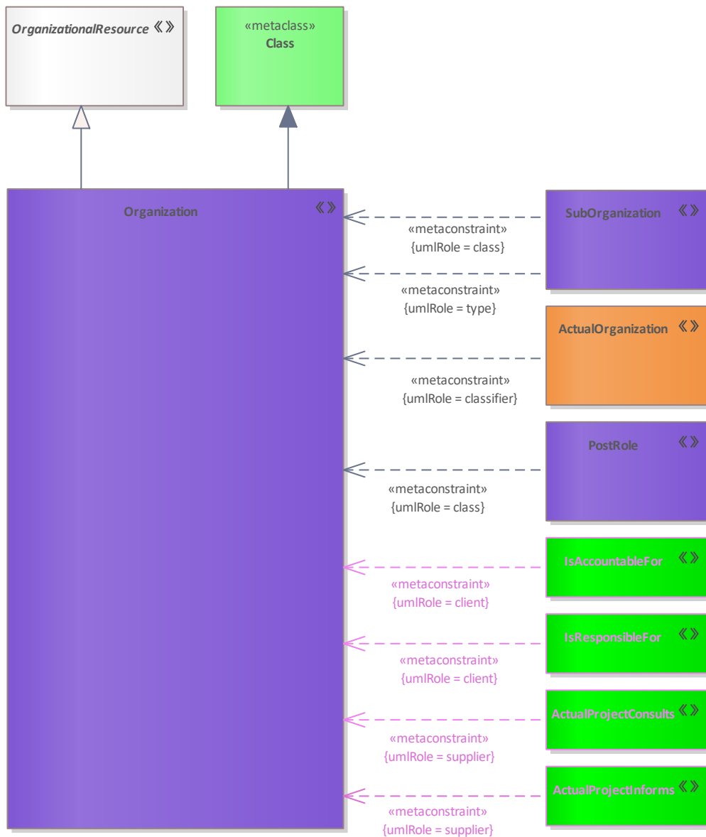
Figure 230: Organization
