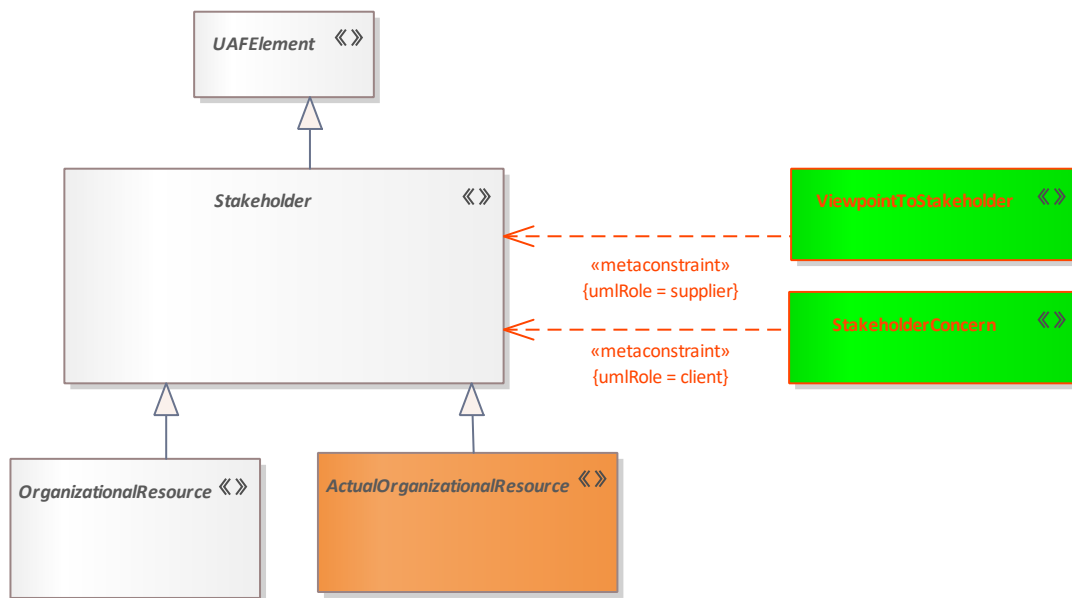
Figure 340: Stakeholder
