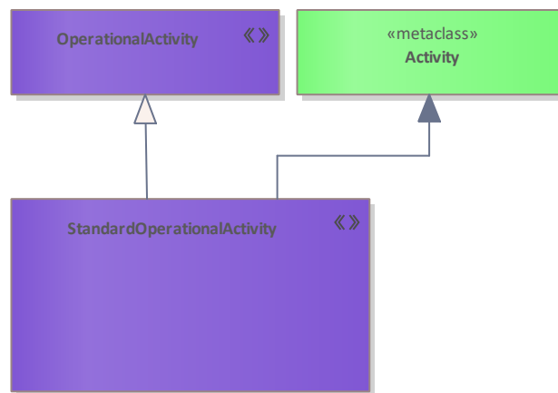
Figure 343: StandardOperationalActivity
