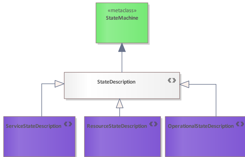
Figure 344: StateDescription
