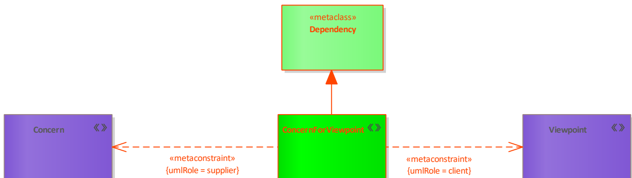
Figure 129: ConcernForViewpoint
