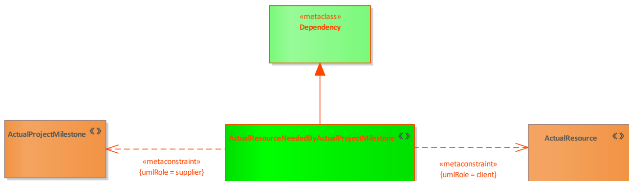
Figure 84: ActualResourceNeededByActualProjectMilestone
