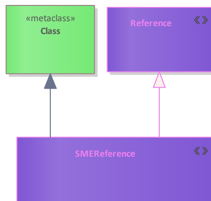
Figure 338: SMEReference
