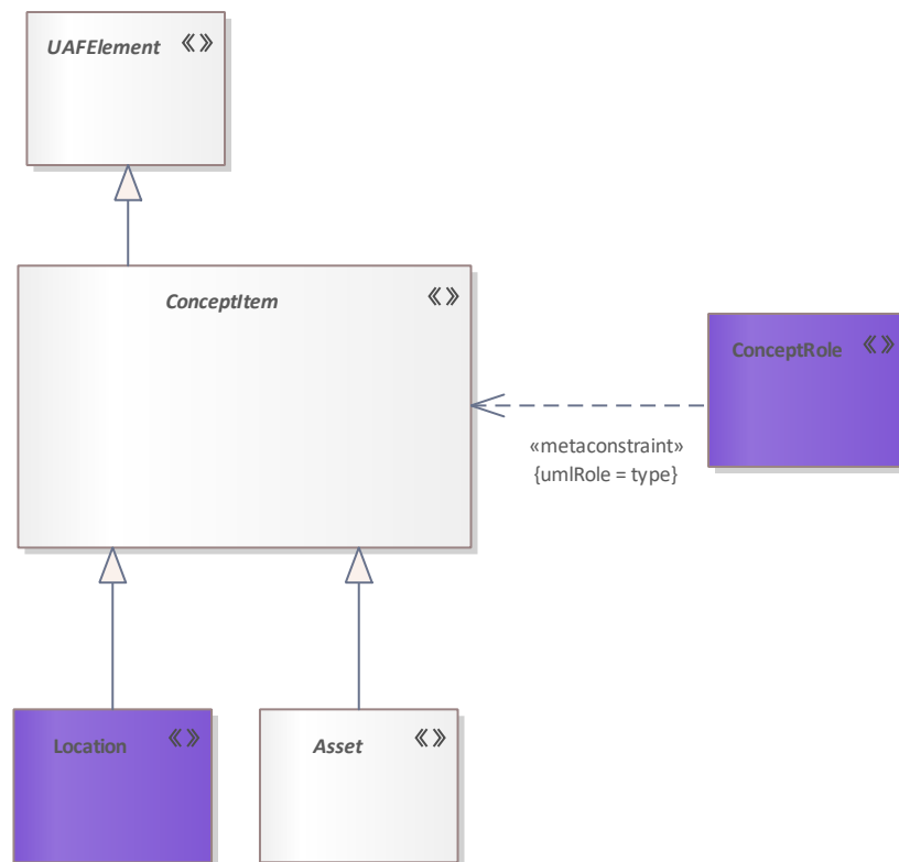
Figure 124: ConceptItem
