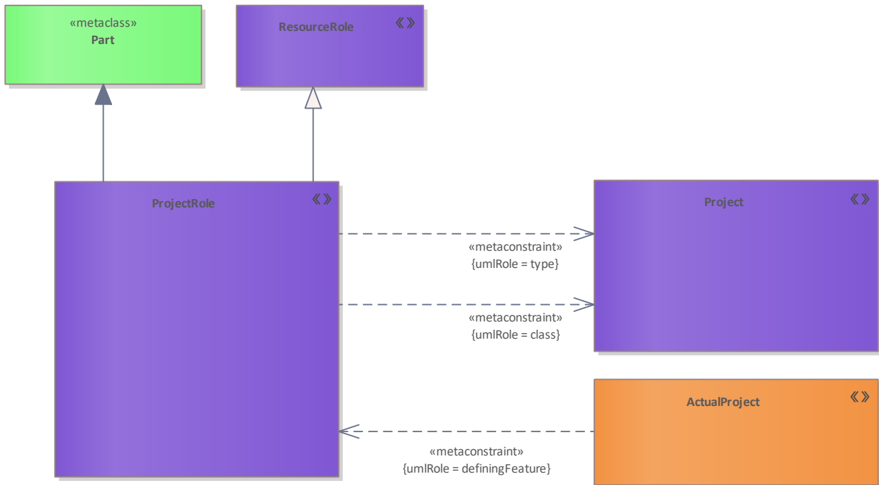
Figure 259: ProjectRole
