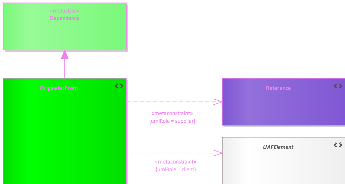
Figure 232: OriginatesFrom
