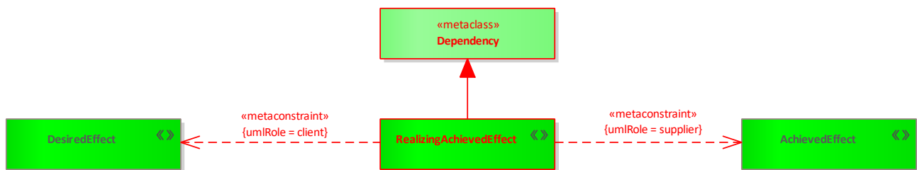
Figure 278: RealizingAchievedEffect
