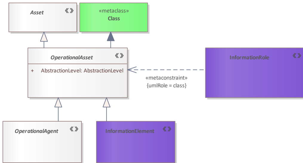
Figure 212: OperationalAsset
