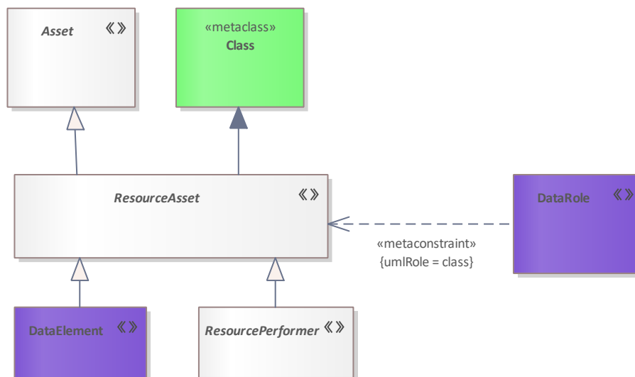
Figure 295: ResourceAsset
