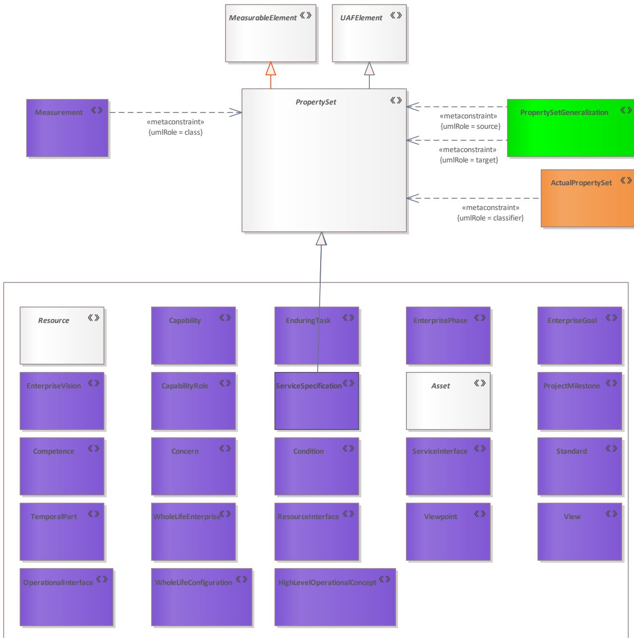
Figure 264: PropertySet
