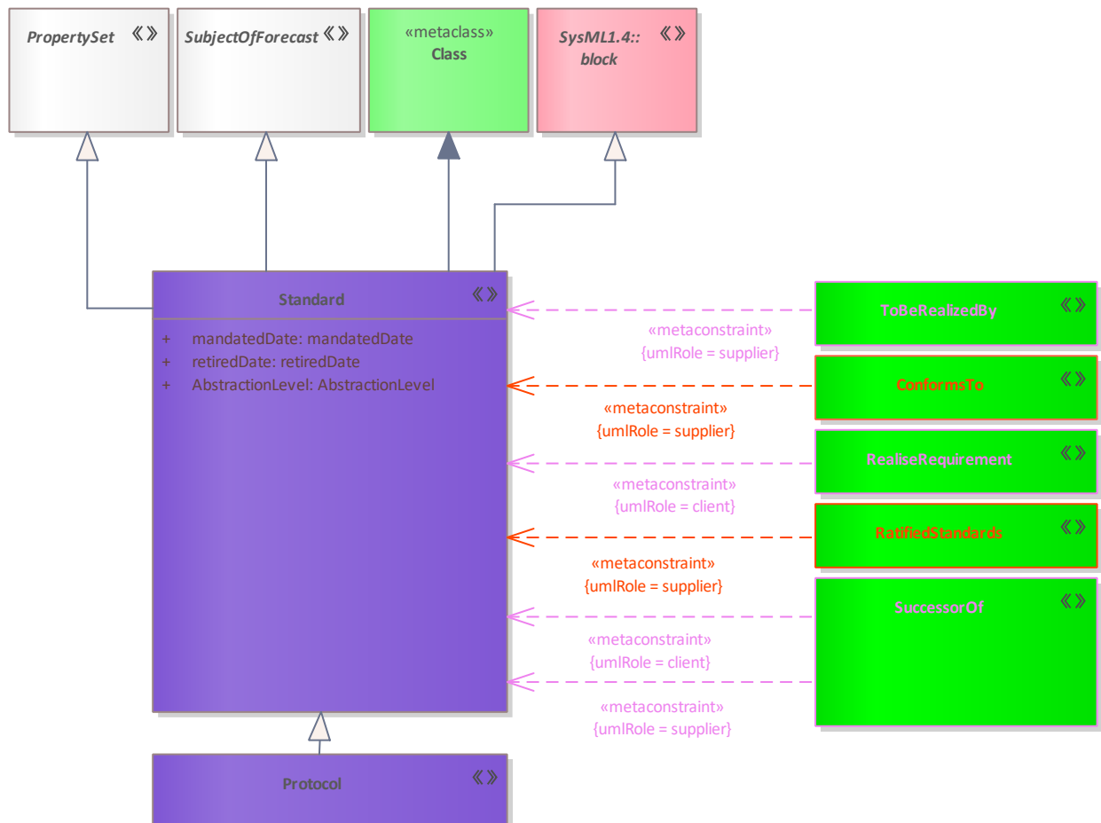
Figure 342: Standard
