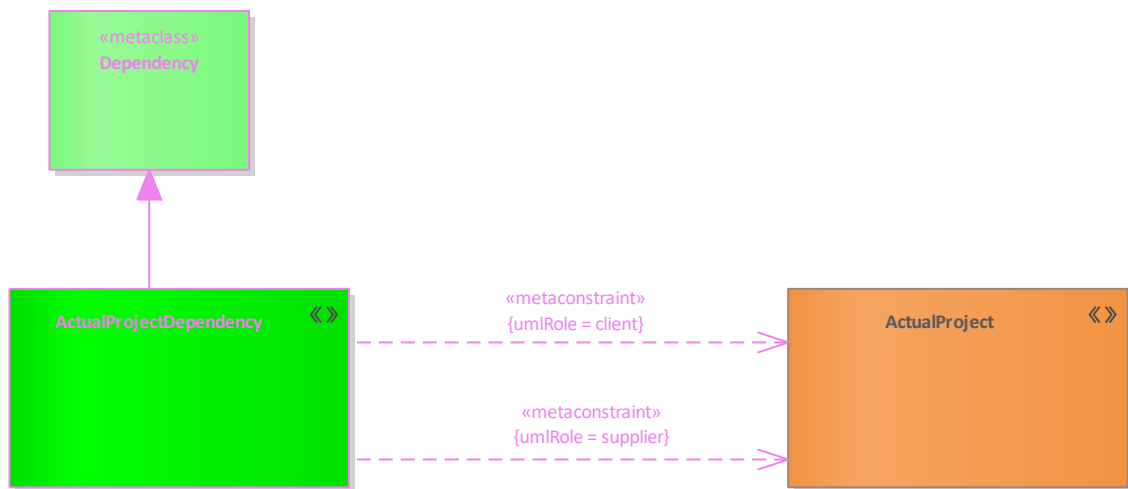
Figure 78: ActualProjectDependency
