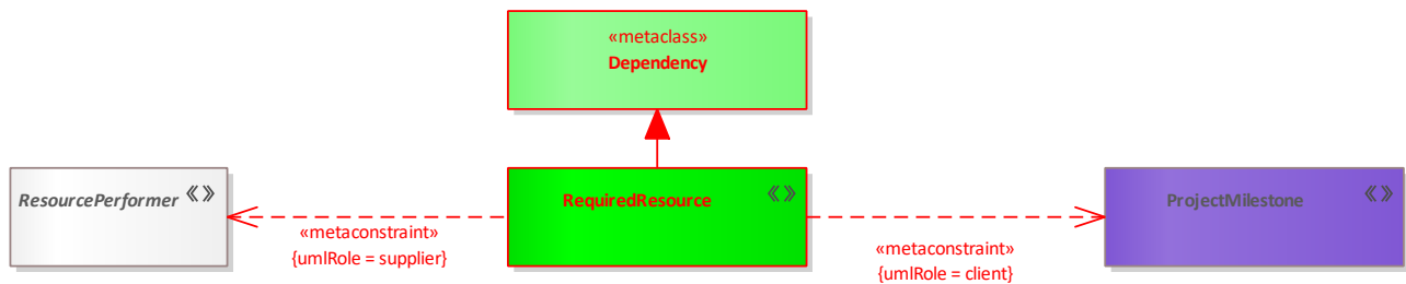
Figure 286: RequiredResource
