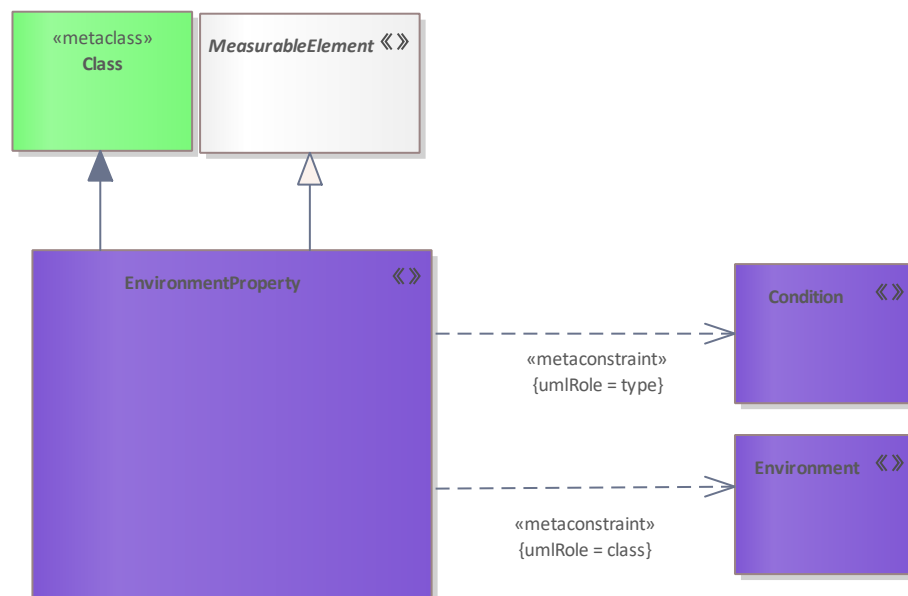
Figure 153: EnvironmentProperty
