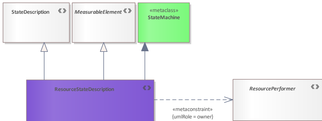
Figure 311: ResourceStateDescription
