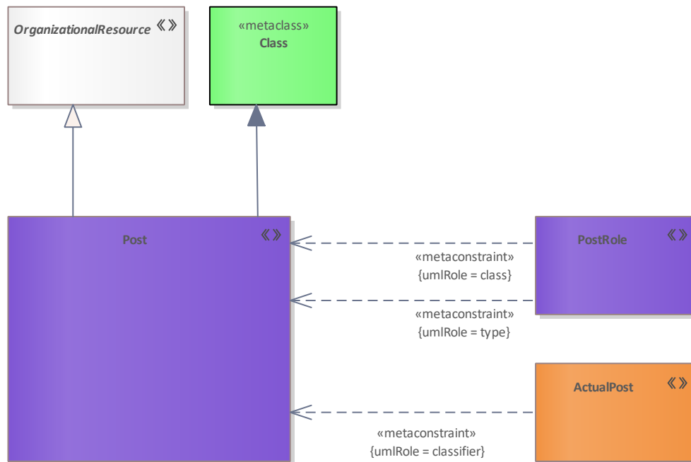
Figure 245: Post
