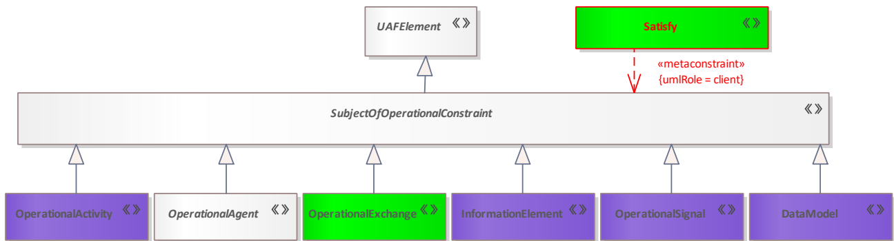
Figure 350: SubjectOfOperationalConstraint
