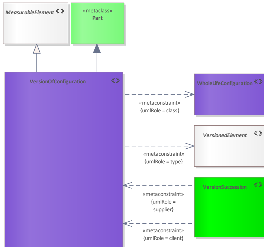
Figure 361: VersionOfConfiguration
