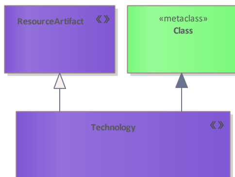
Figure 356: Technology
