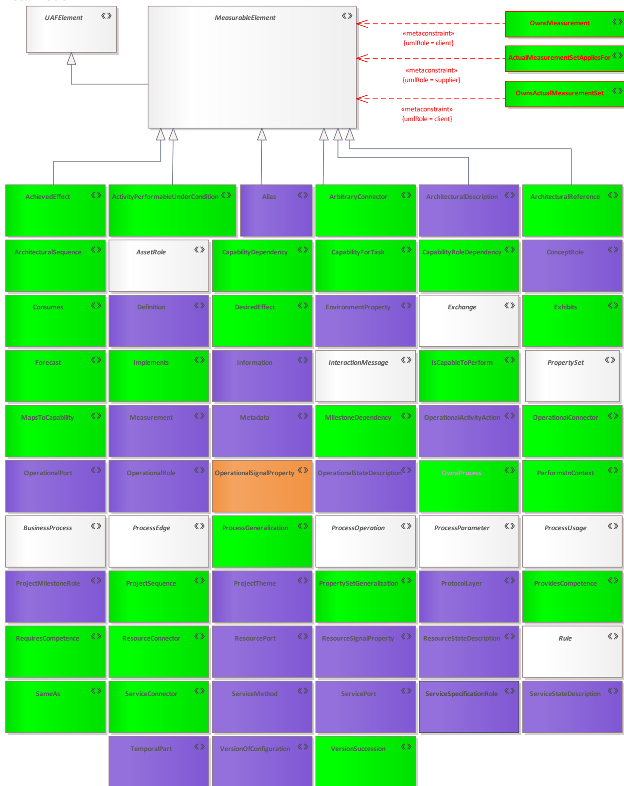
Figure 196: MeasurableElement
