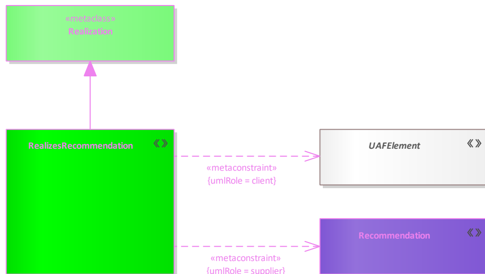
Figure 277: RealizesRecommendation
