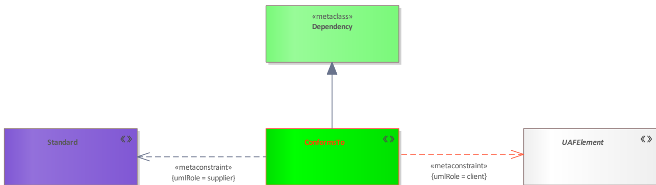
Figure 132: ConformsTo
