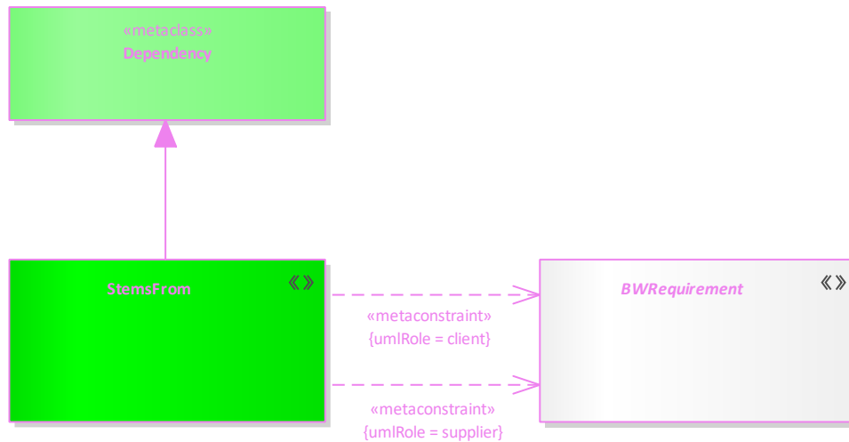
Figure 346: StemsFrom
