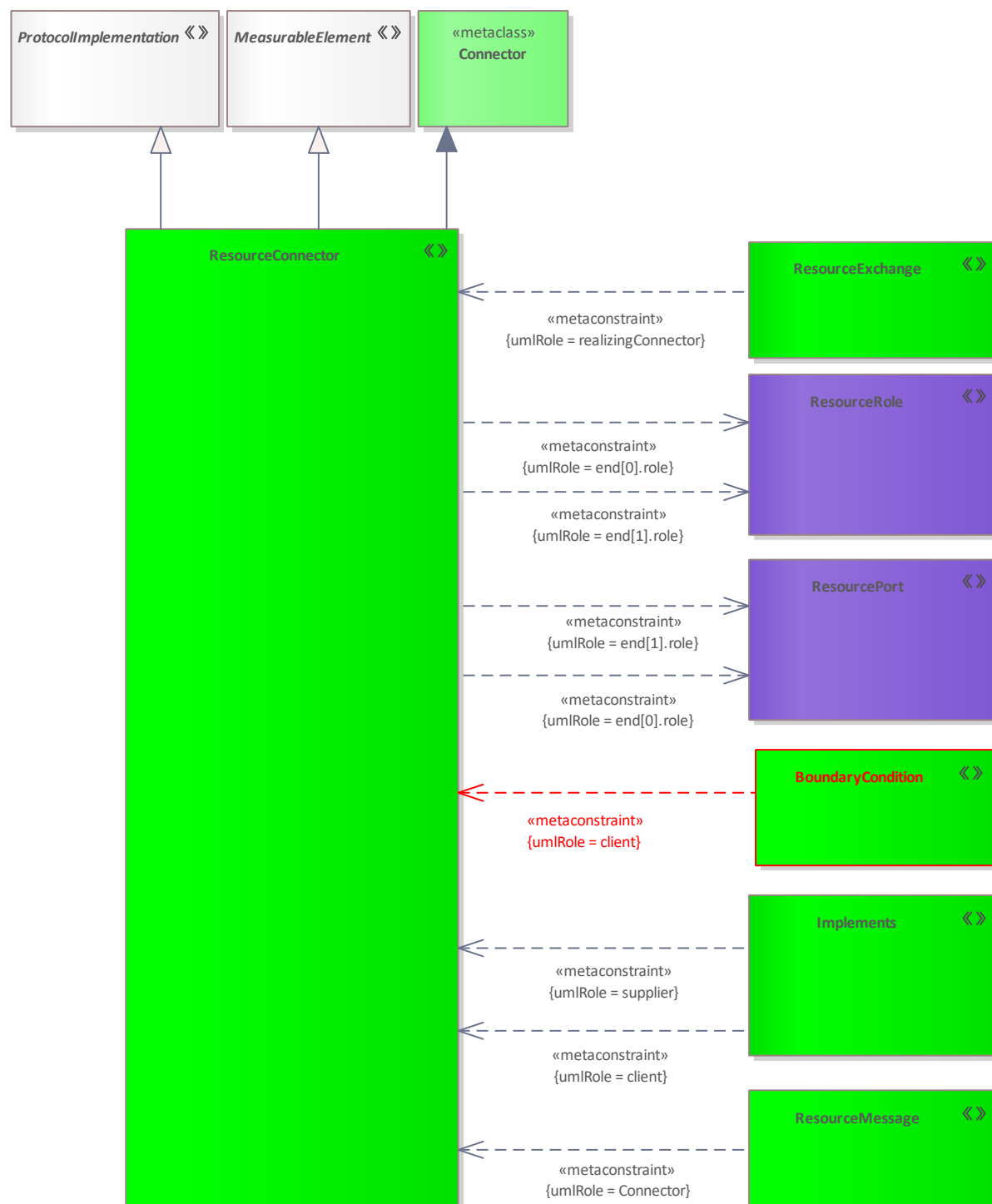
Figure 296: ResourceConnector
