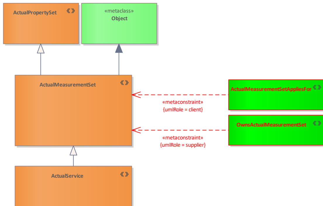
Figure 69: ActualMeasurementSet
