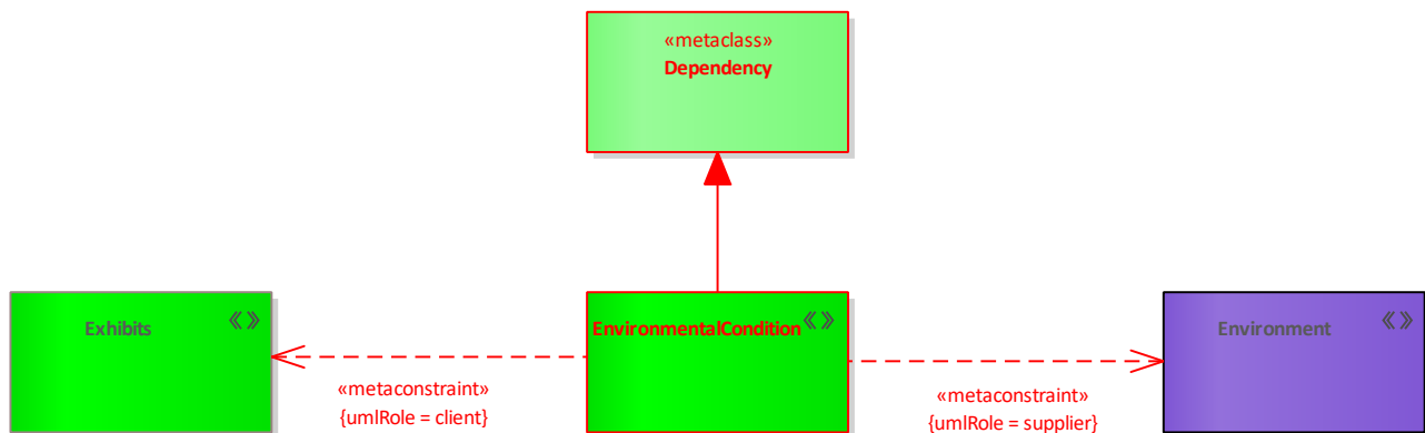
Figure 151: EnvironmentalCondition
