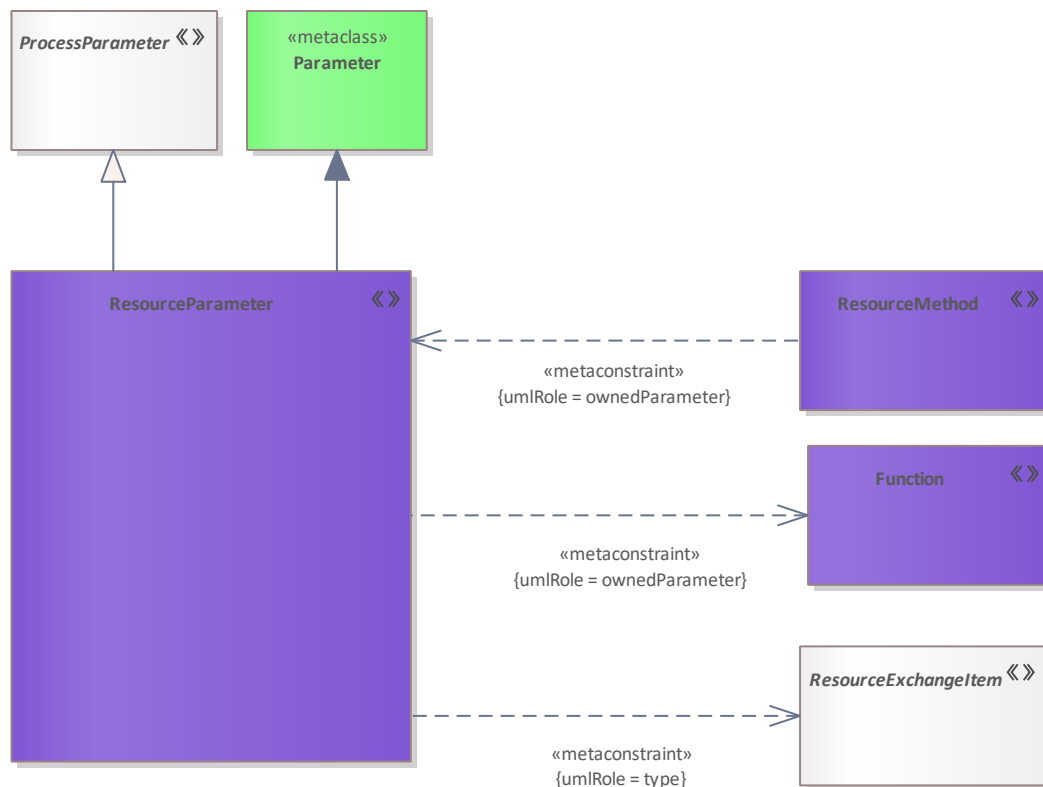
Figure 305: ResourceParameter
