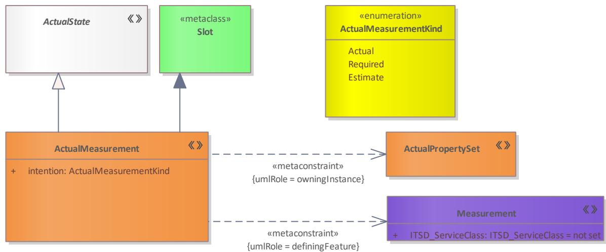
Figure 68: ActualMeasurement
