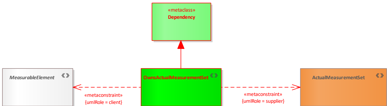
Figure 234: OwnsActualMeasurementSet
