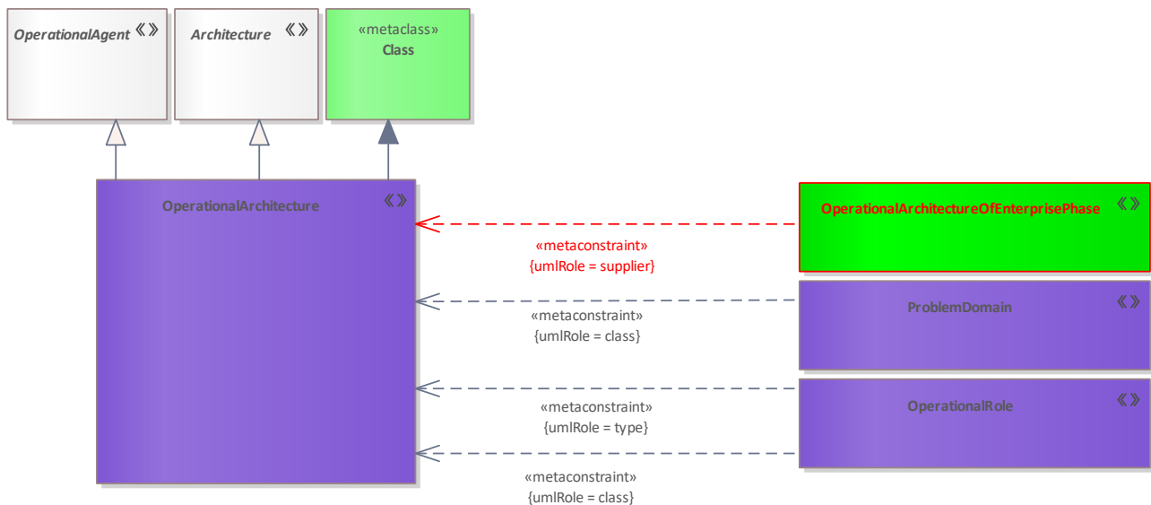
Figure 210: OperationalArchitecture
