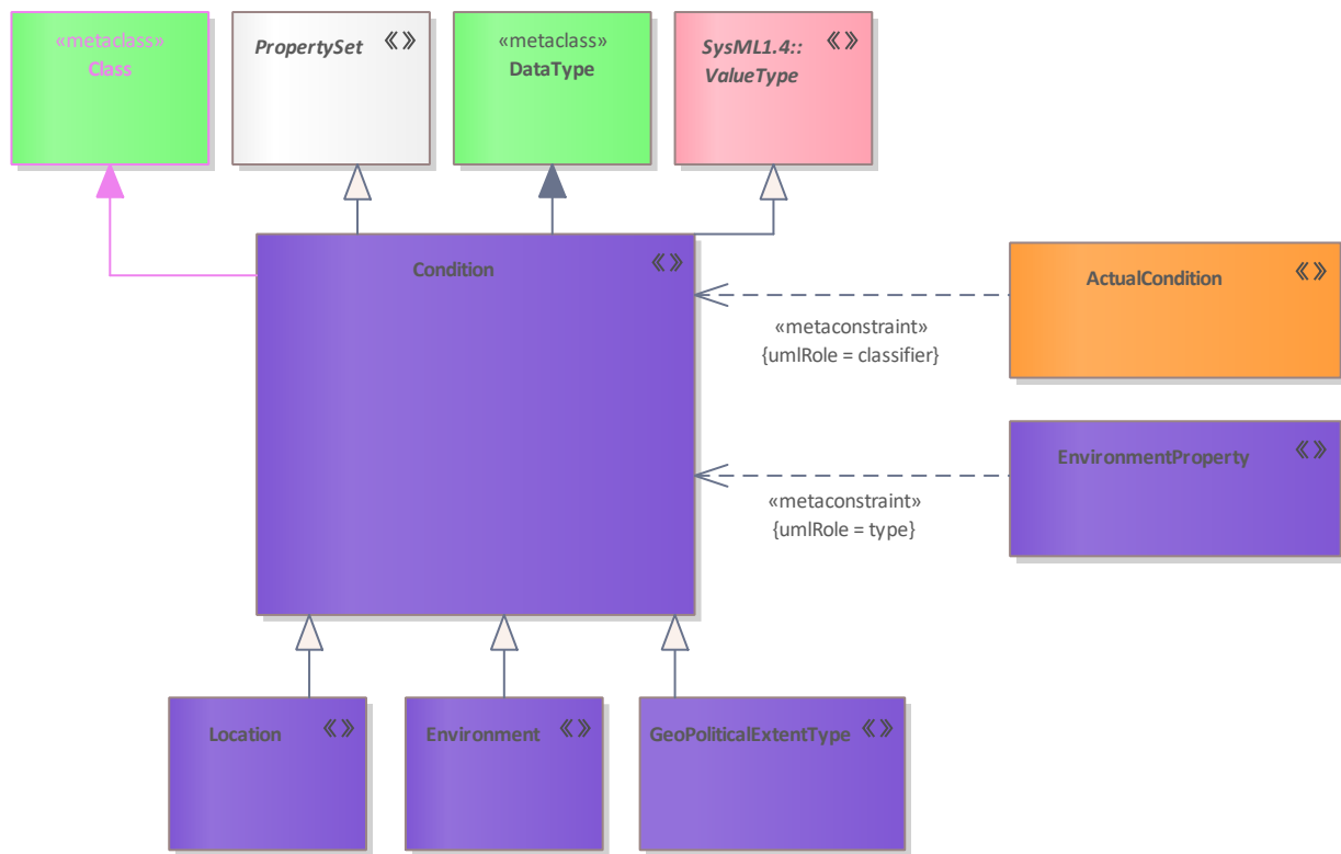
Figure 130: Condition
