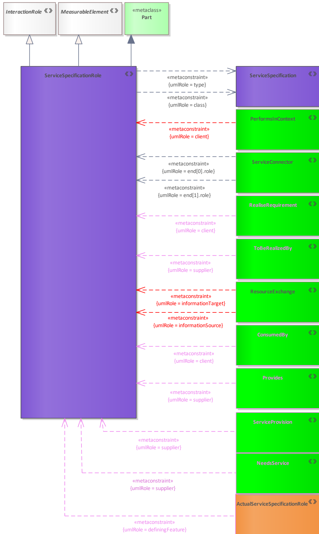
Figure 336: ServiceSpecificationRole
