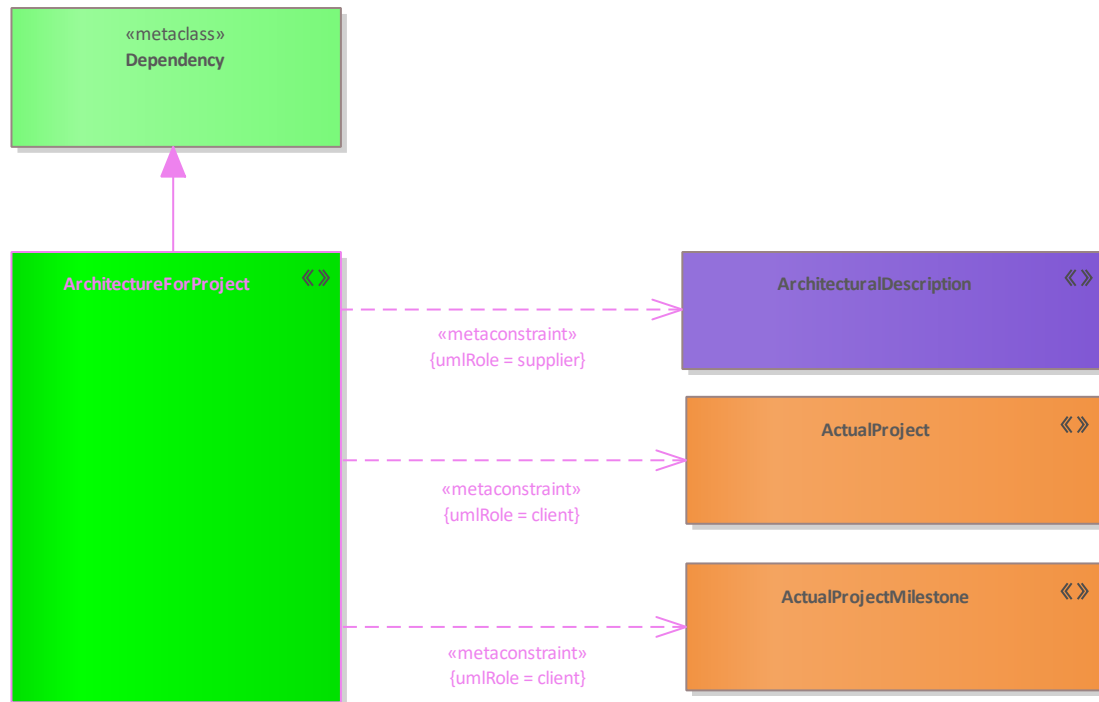
Figure 102: ArchitectureForProject
