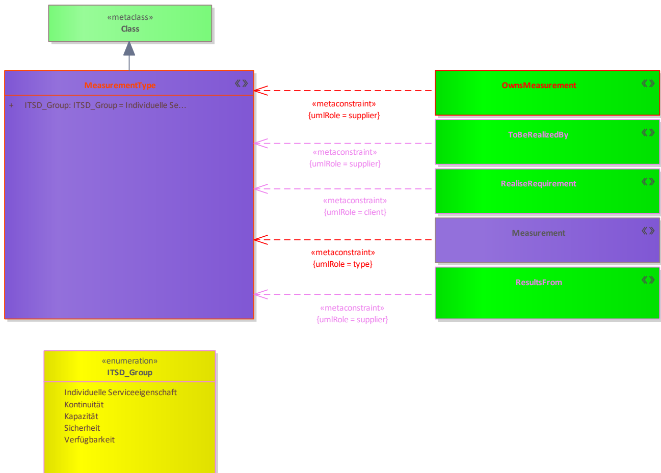
Figure 198: MeasurementType
