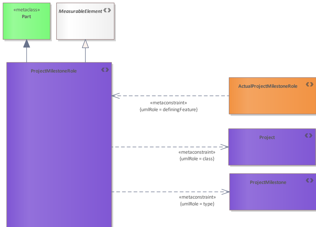
Figure 256: ProjectMilestoneRole
