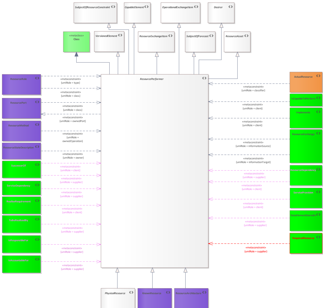
Figure 306: ResourcePerformer
