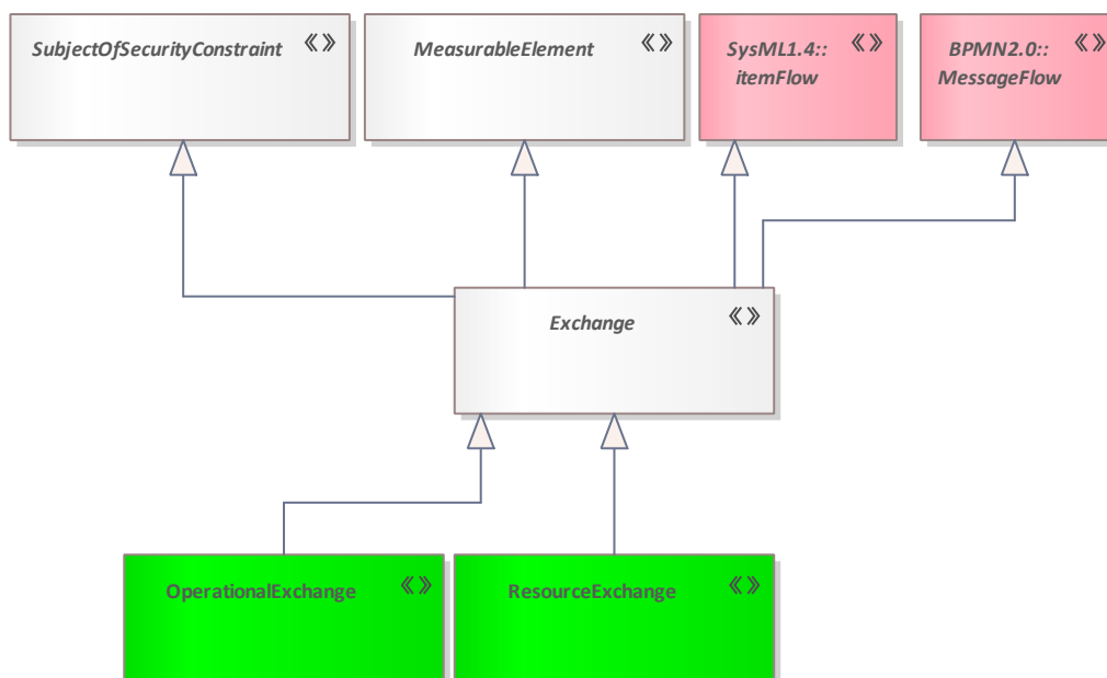
Figure 155: Exchange
