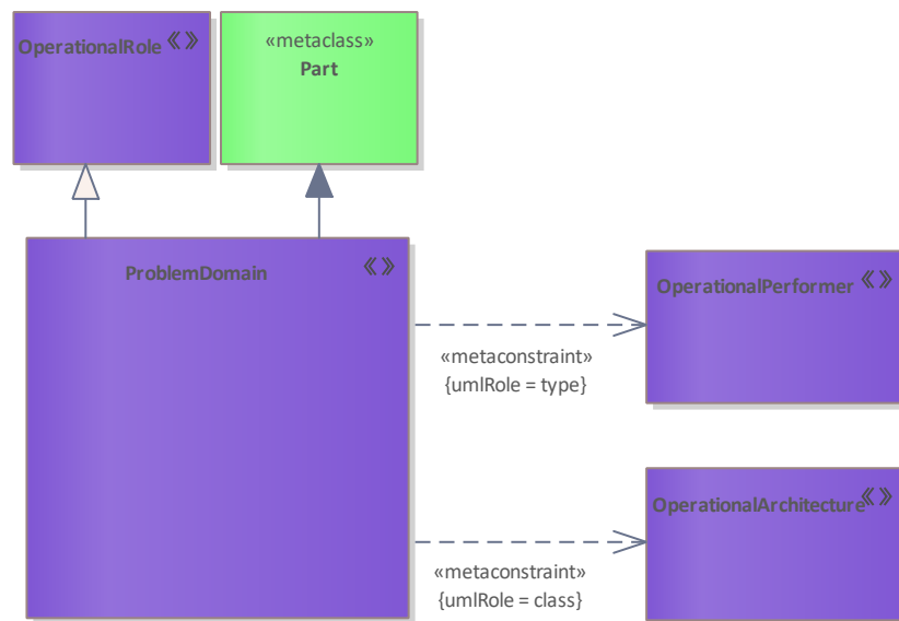
Figure 247: ProblemDomain
