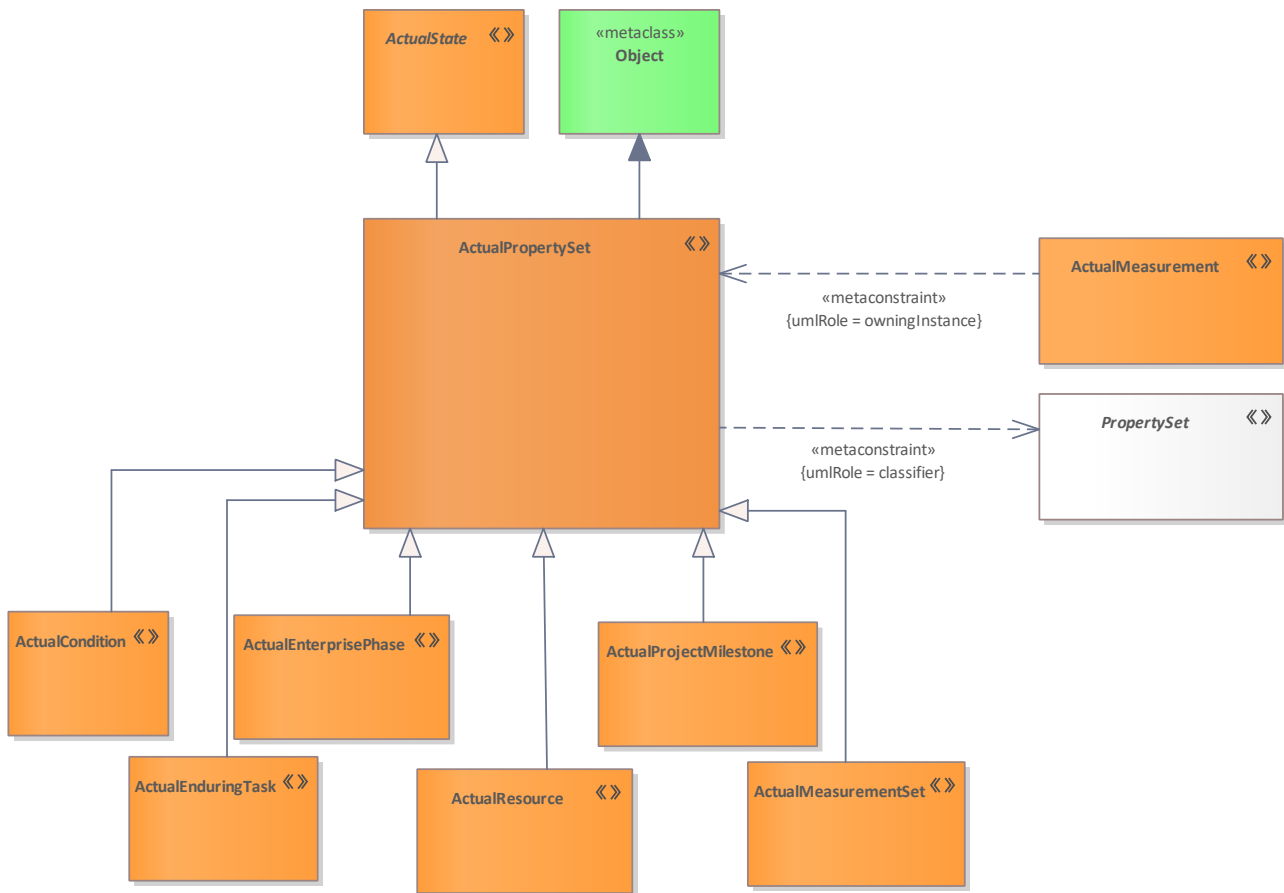
Figure 82: ActualPropertySet
