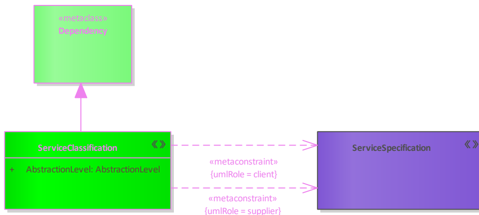
Figure 322: ServiceClassification
