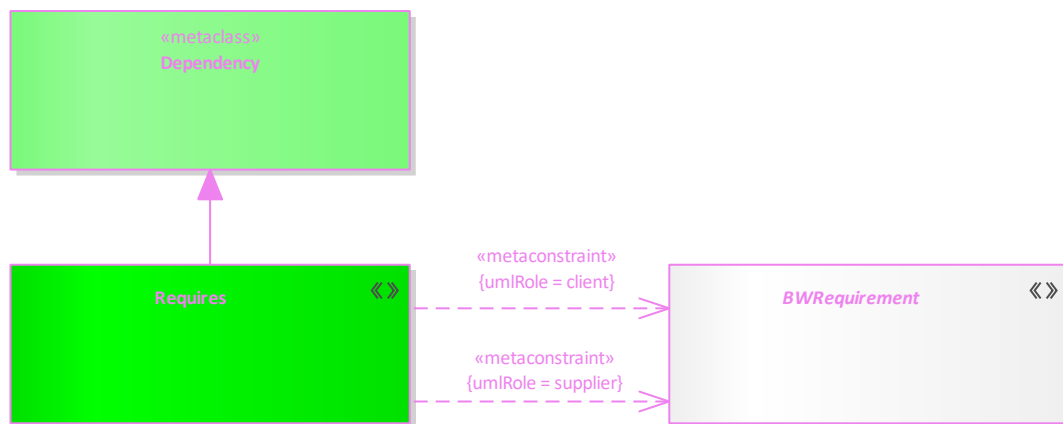
Figure 290: Requires
