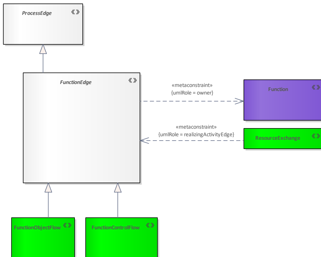
Figure 171: FunctionEdge
