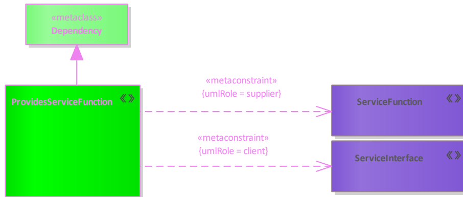
Figure 273: ProvidesServiceFunction
