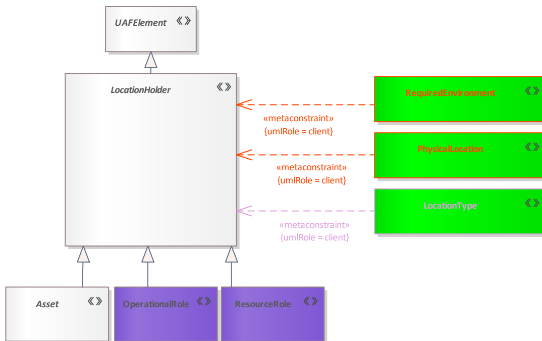
Figure 193: LocationHolder
