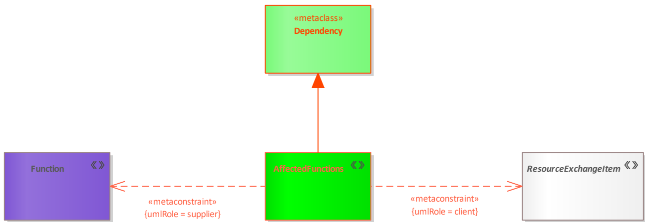
Figure 93: AffectedFunctions
