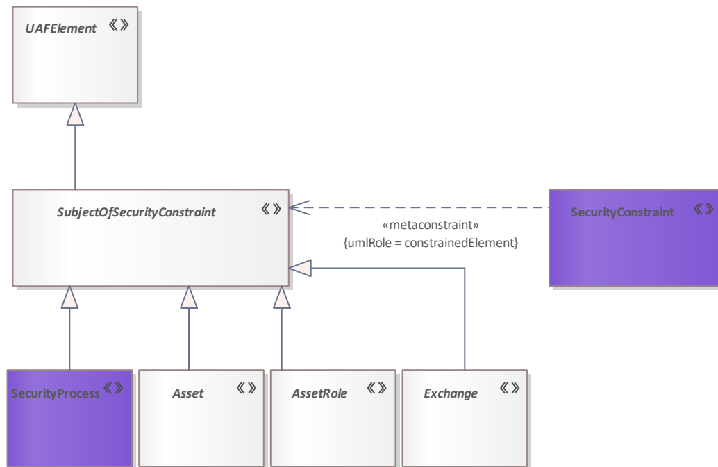
Figure 352: SubjectOfSecurityConstraint
