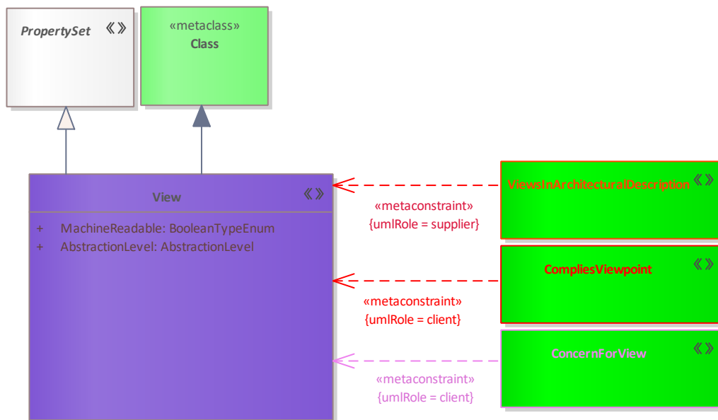
Figure 365: View
