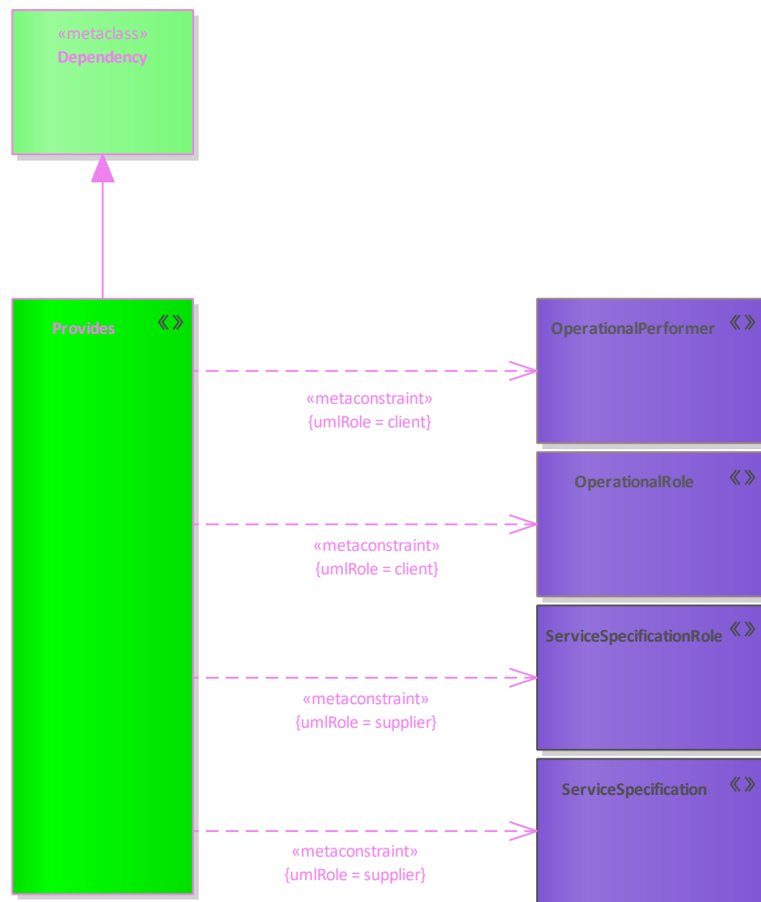
Figure 271: Provides
