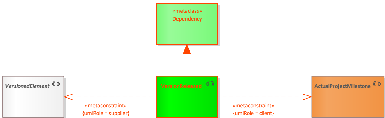
Figure 362: VersionReleased
