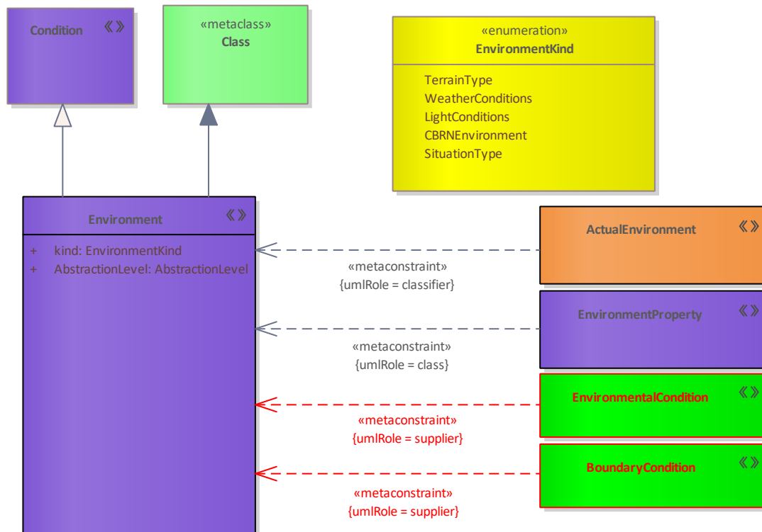
Figure 150: Environment
