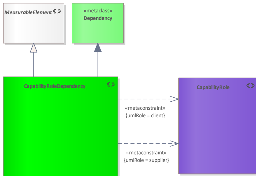
Figure 115: CapabilityRoleDependency
